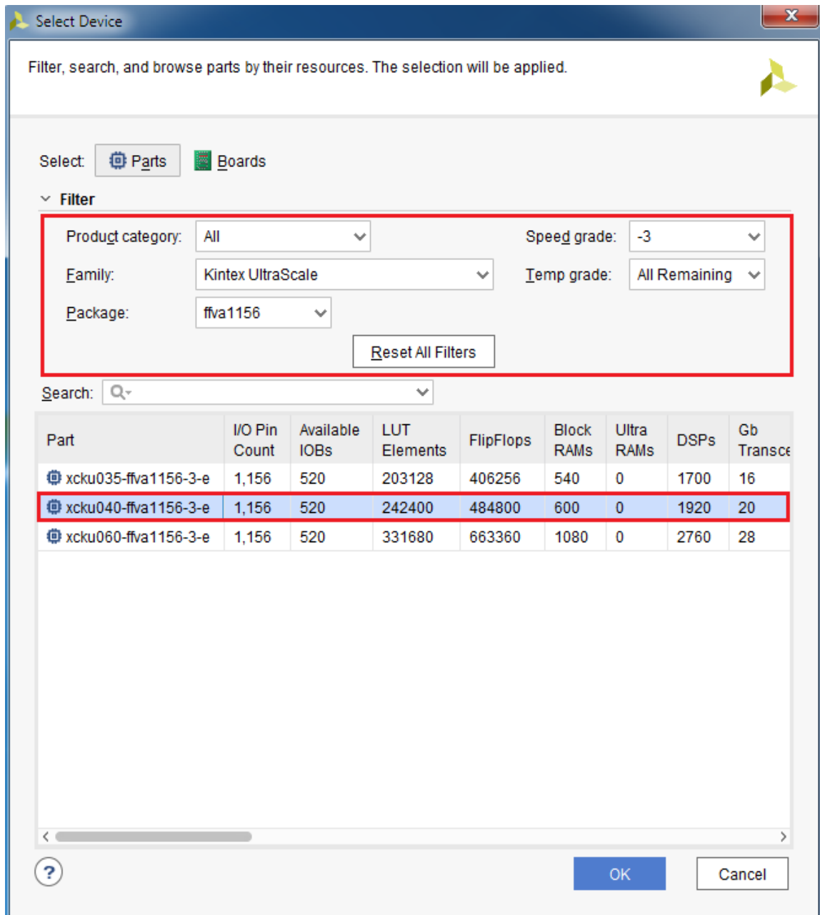
Figure 2-2: Select Device
