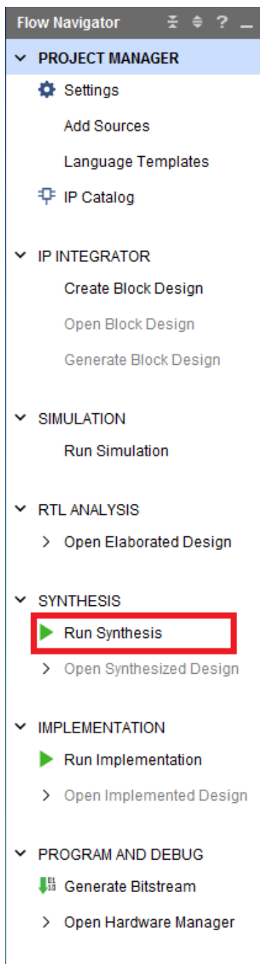
Figure 2-10: Run Synthesis
