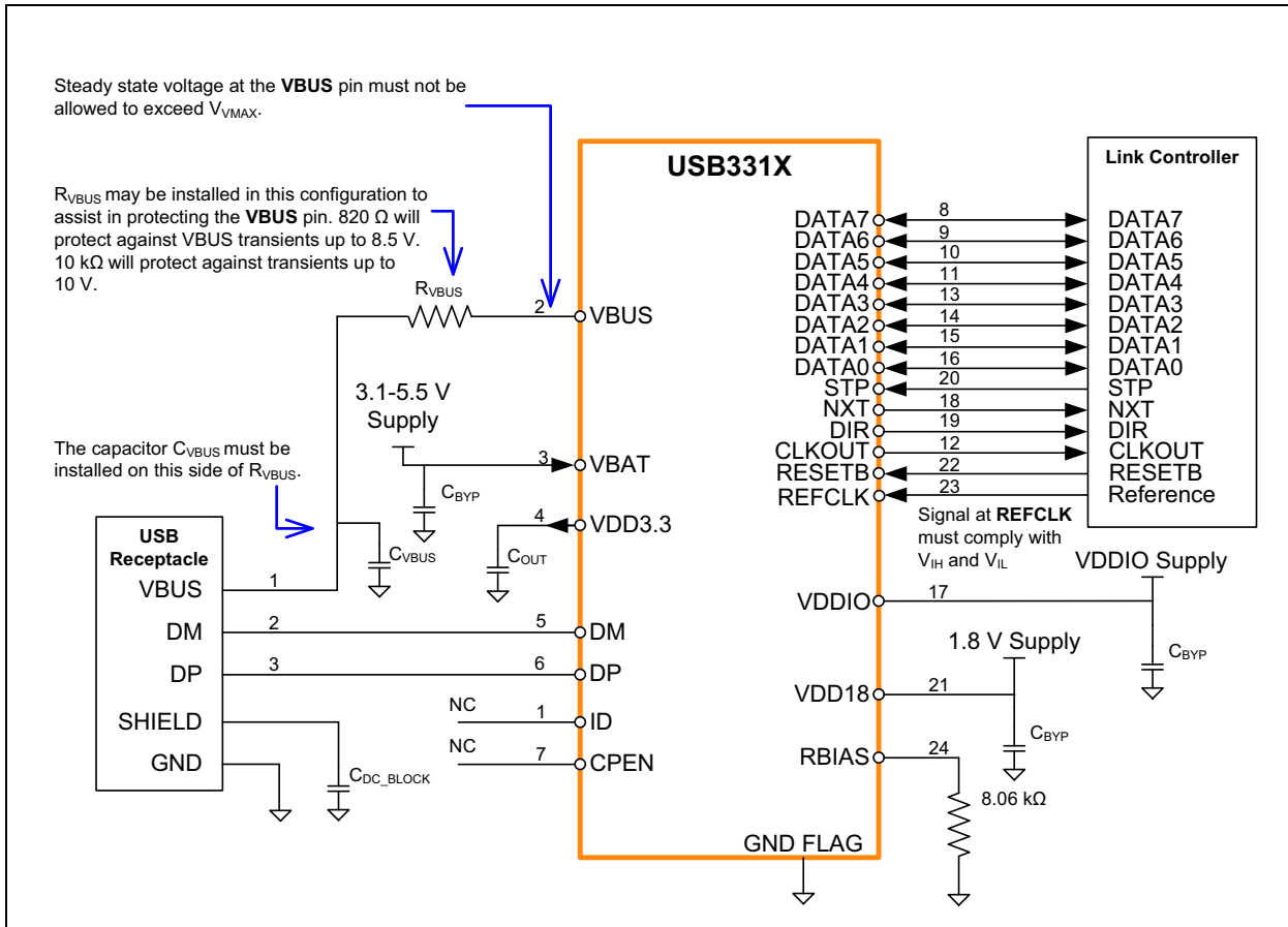
FIGURE 8-1: USB3317 QFN APPLICATION DIAGRAM (DEVICE)
