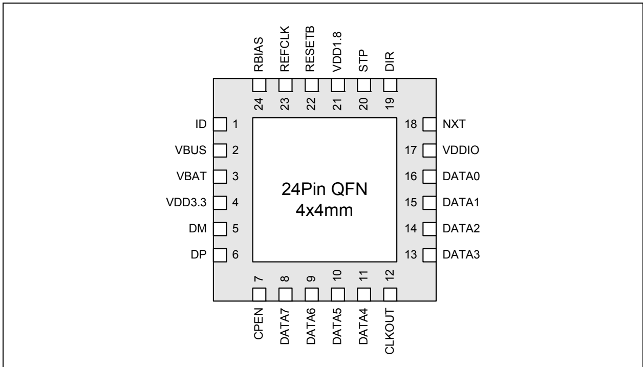
FIGURE 2-1: USB3317 QFN PINOUT - TOP VIEW
