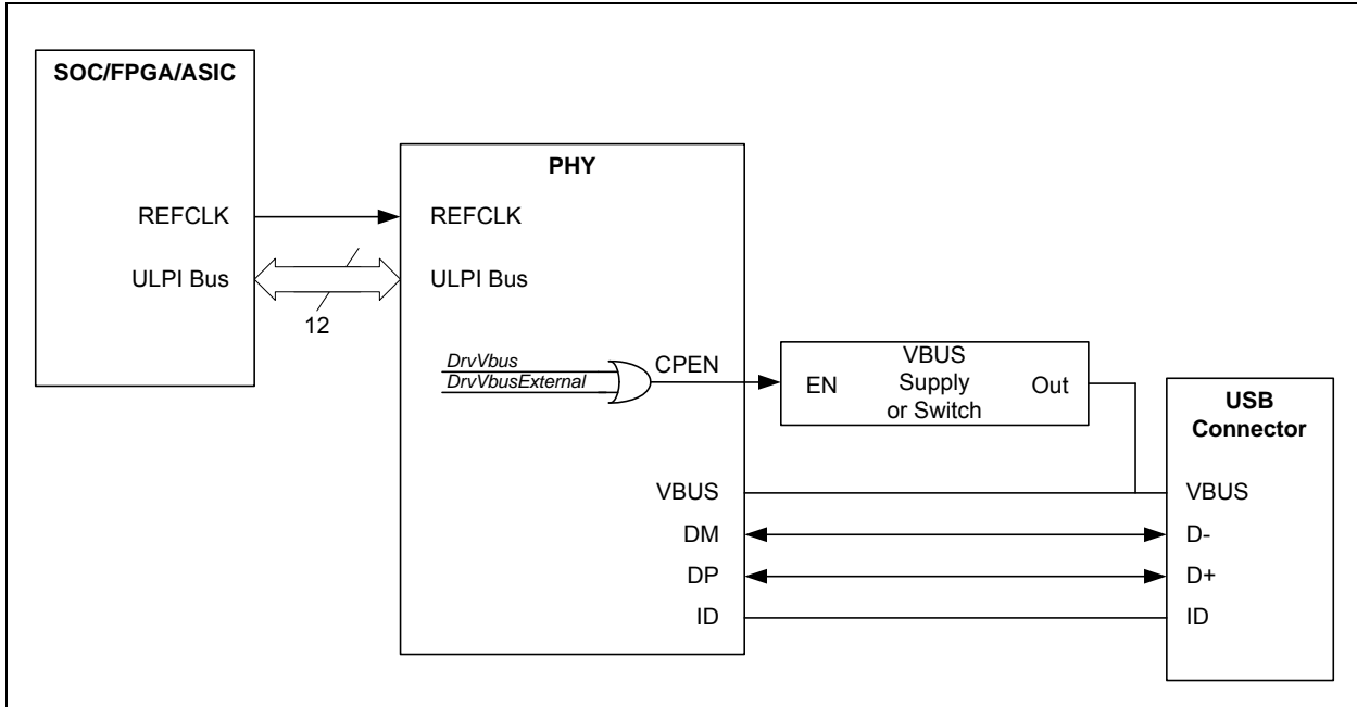
FIGURE 5-9: USB3317 DRIVES EXTERNAL VBUS SUPPLY OR SWITCH
