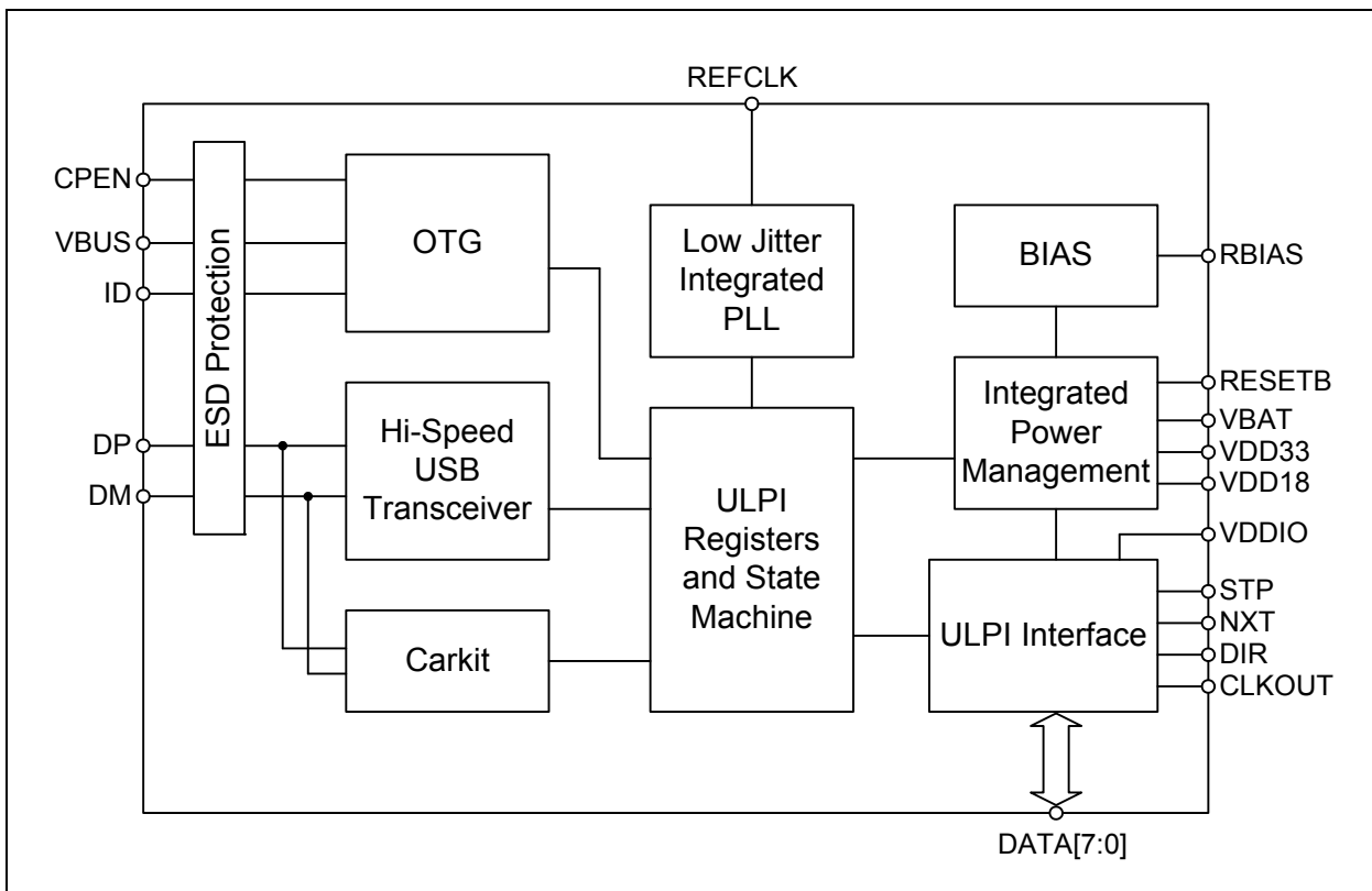
FIGURE 1-1: USB3317 BLOCK DIAGRAM
