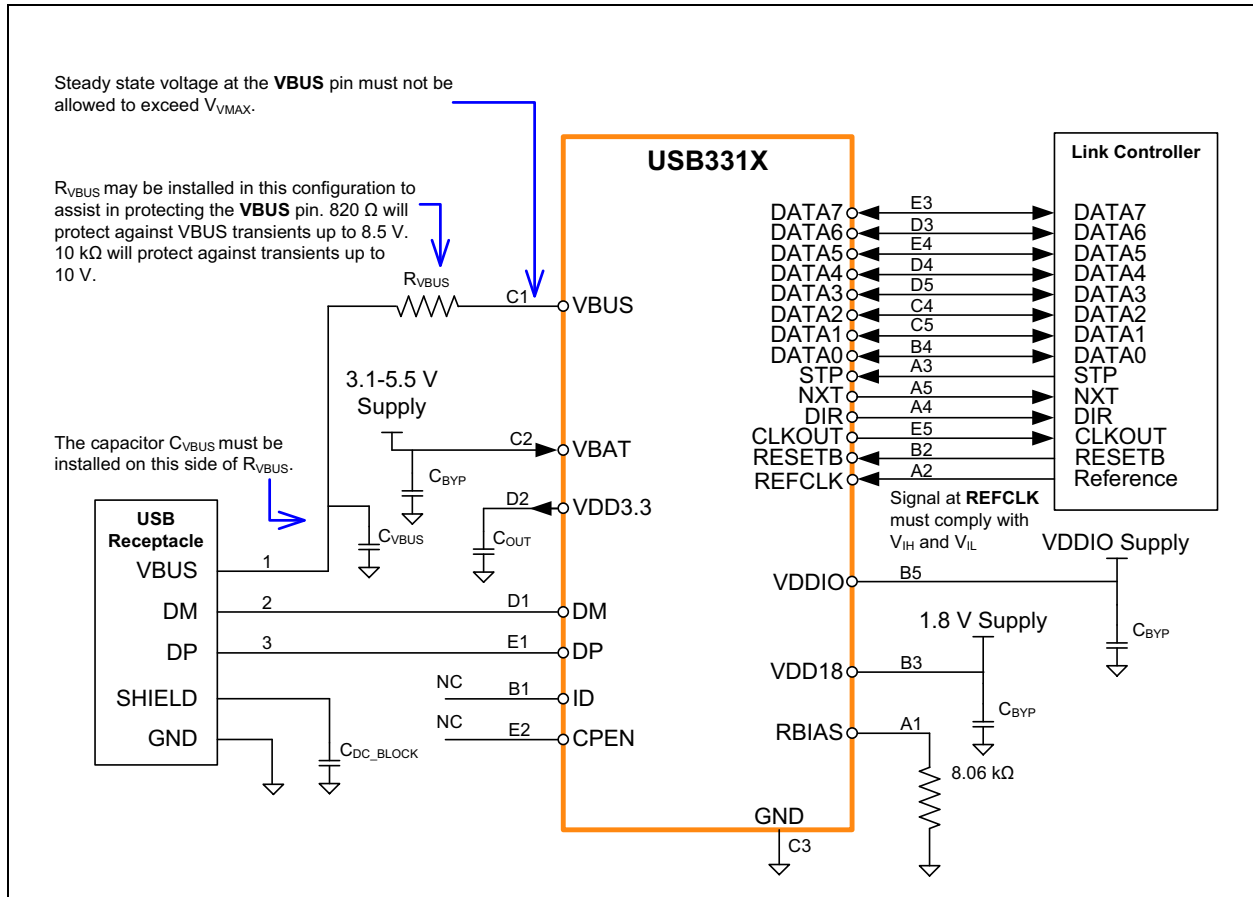
FIGURE 8-2: USB3317 VFBGA APPLICATION DIAGRAM (DEVICE)
