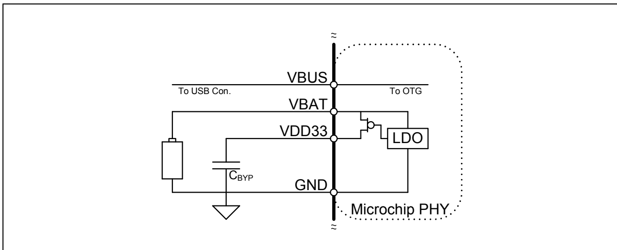
FIGURE 5-3: POWERING THE USB3317 FROM A BATTERY
