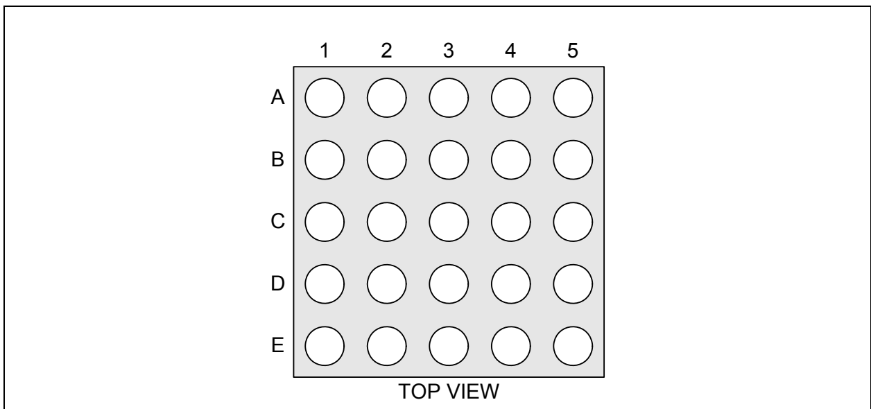
FIGURE 2-2: USB3317 VFBGA PINOUT - TOP VIEW
