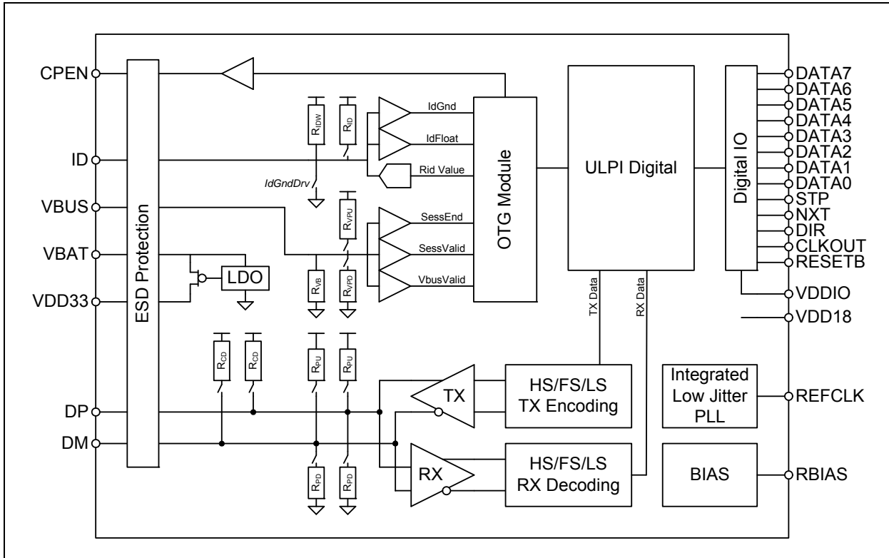
FIGURE 5-1: USB3317 SYSTEM DIAGRAM
