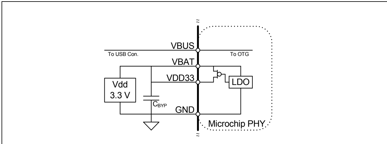
FIGURE 5-4: POWERING THE USB3317 FROM A 3.3 V SUPPLY
