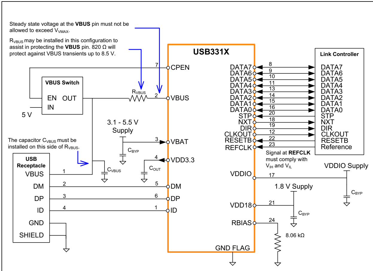
FIGURE 8-3: USB3317 QFN APPLICATION DIAGRAM (HOST OR OTG)
