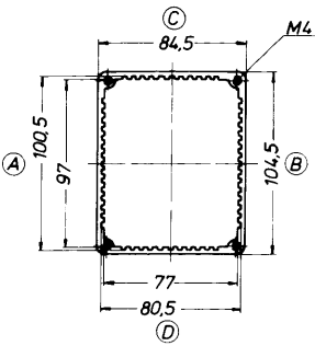
Profile Type 07.05 / L = 125 mm
