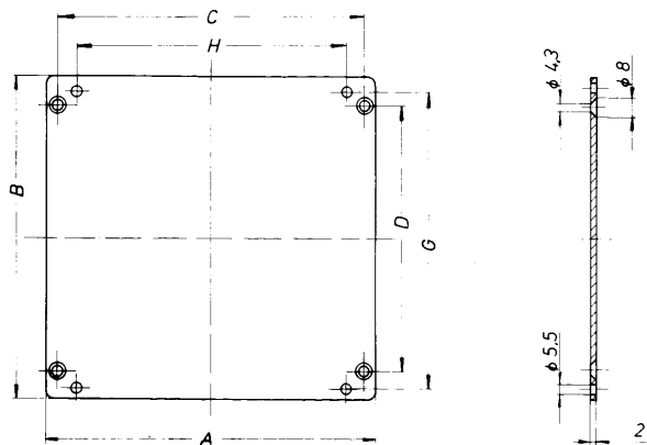
Flat aluminium rear wall mounting
