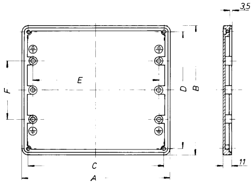
Aluminium cast lid
