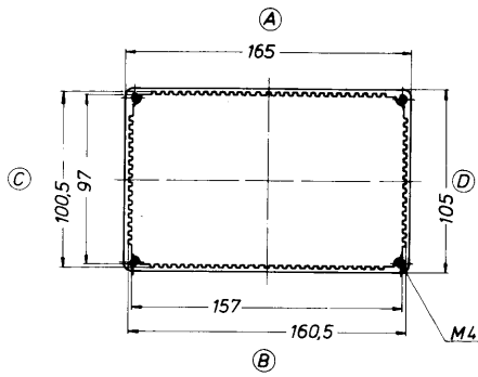
Profile Type 07.06 / L = 180 mm
