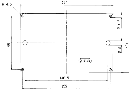
Front plate for membrane lid Type 07.06
