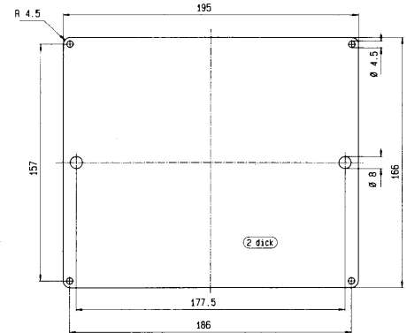
Front plate for membrane lid Type 07.07
