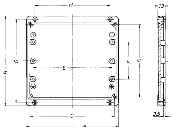
Cast aluminium rear wall mounting
