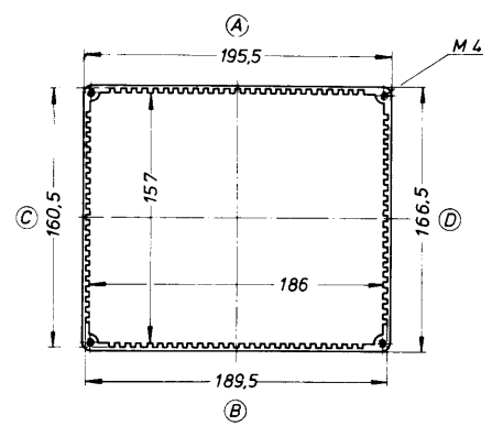
Profile Type 07.07 / L = 180 mm
