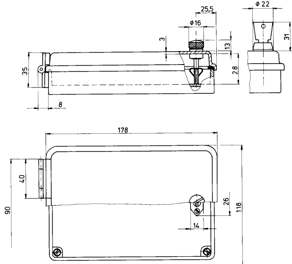
Transparent cover for cast aluminium bezel lid
