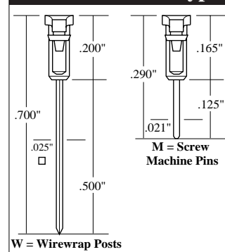
Bottom Male Pin Types
