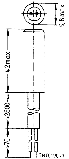
Dimensions in mm Approx. weight 80 g
