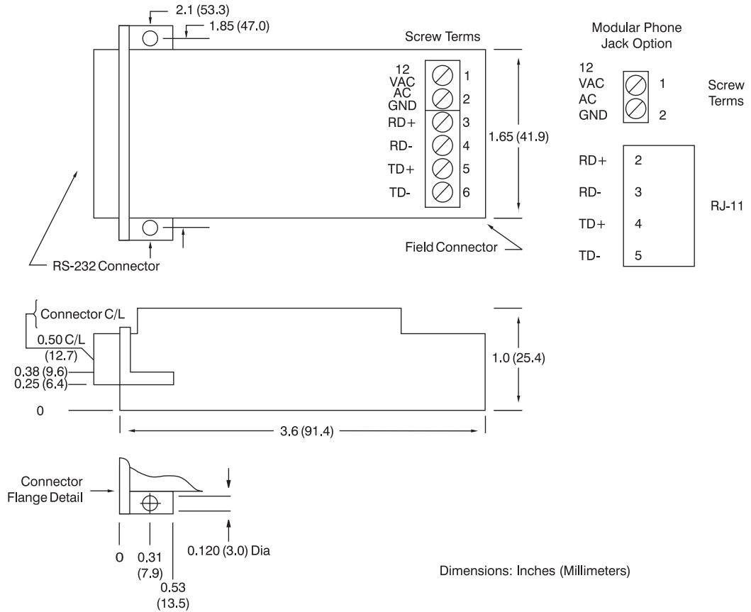
Figure 3. LDM30 Mechanical Drawing
