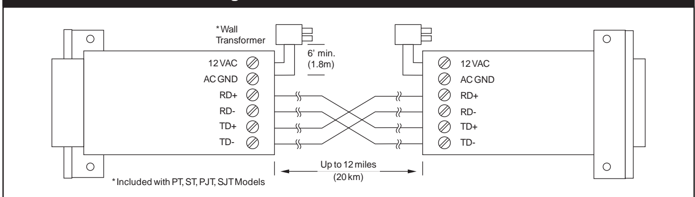
Figure 2. LDM30 Field Connections
