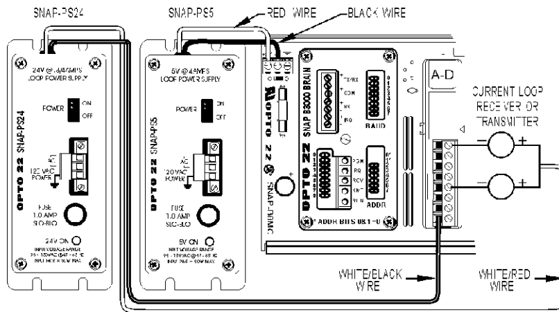
FIGURE 2-SNAP-PS24
