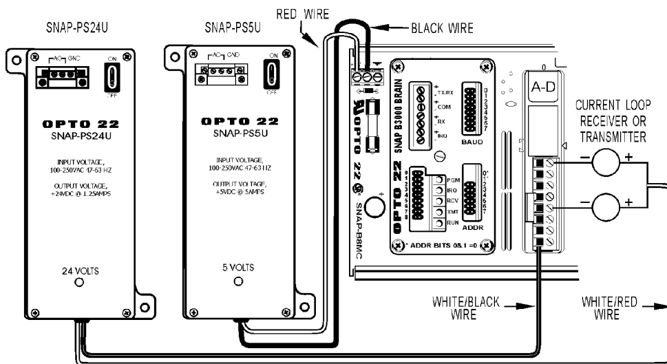
FIGURE 2 - SNAP-PS24U
