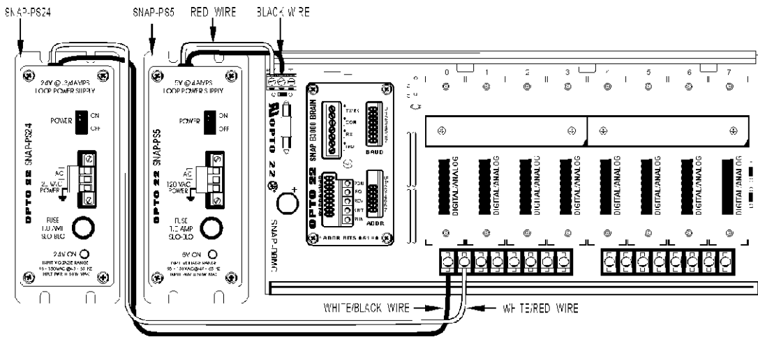
FIGURE 2-SNAP-PS24
