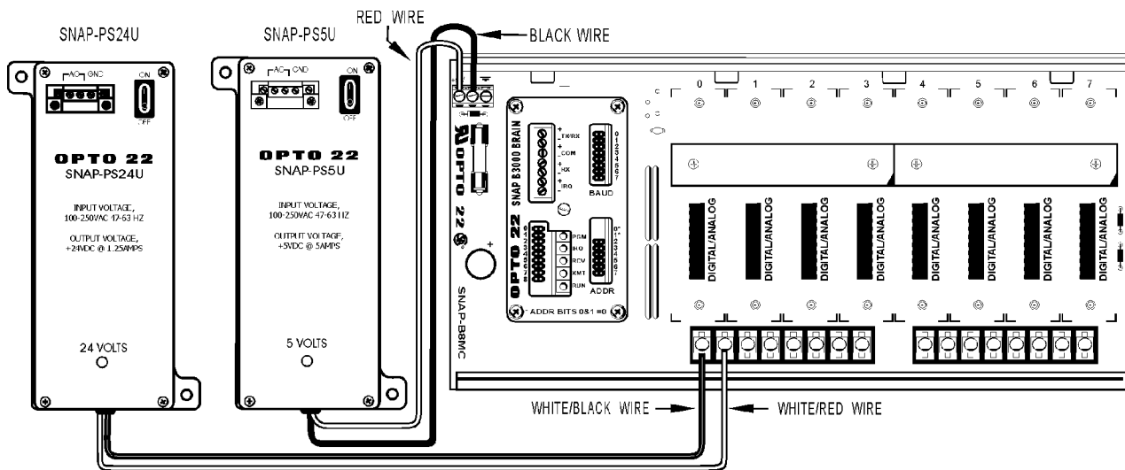
FIGURE 1 - SNAP-PS24U
