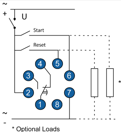
MDE1...24U
