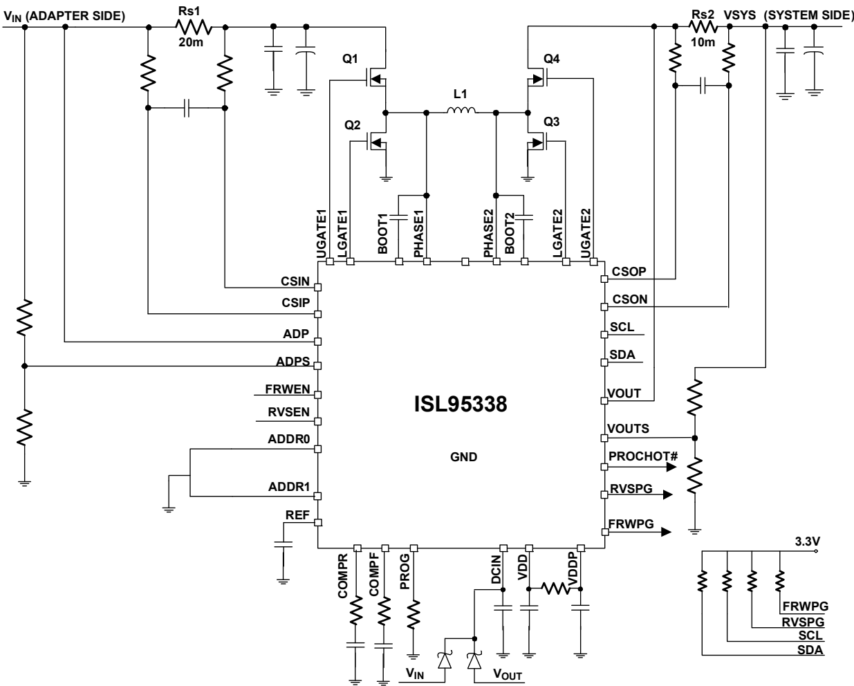
Figure 3. Simplified Application Diagram
