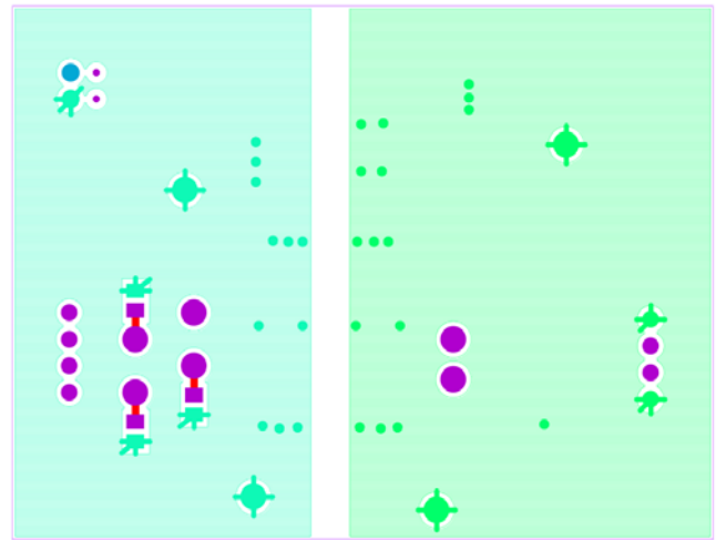
Figure 8. Bottom Layer
