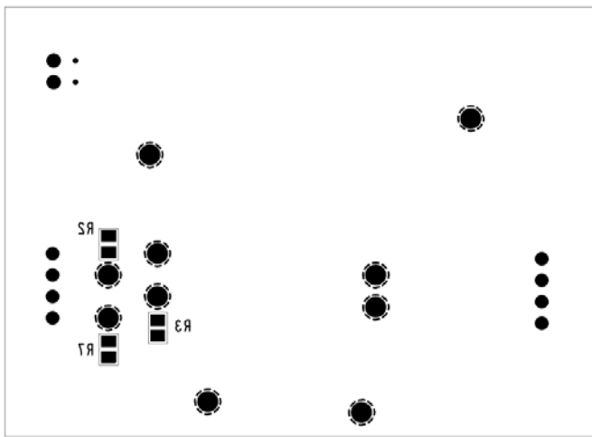
Figure 7. Silkscreen Bottom
