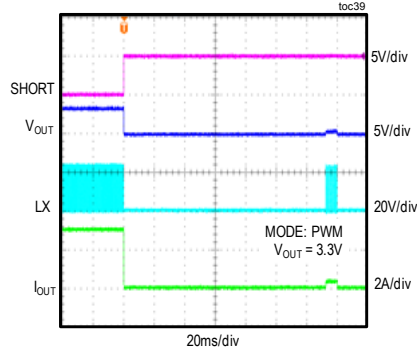
OUTPUT SHORT IN STEADY STATE (LOAD CURRENT 3A)
