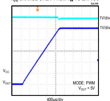
V_{CC} CHANGE OVER FROM V_{IN} TO EXT V_{CC}
