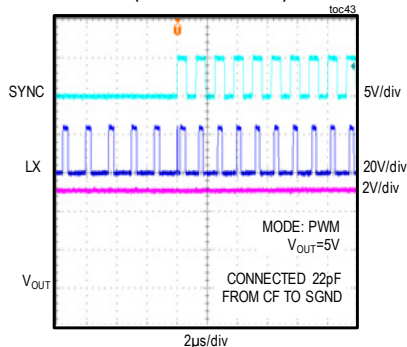
EXTERNAL SYNCHRONIZATION (LOAD CURRENT 3A)
