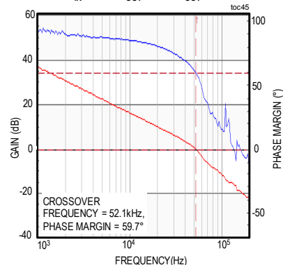
BODE PLOT
