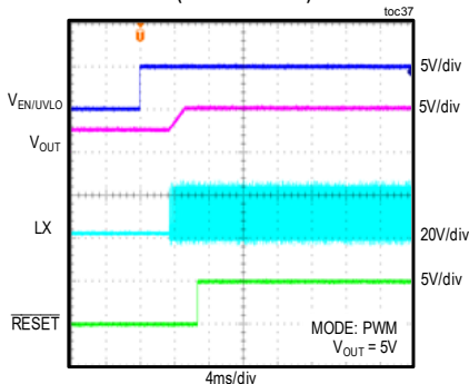
START-UP INTO PREBIAS 2.5V TO V_O = 5V (NO-LOAD PWM)
