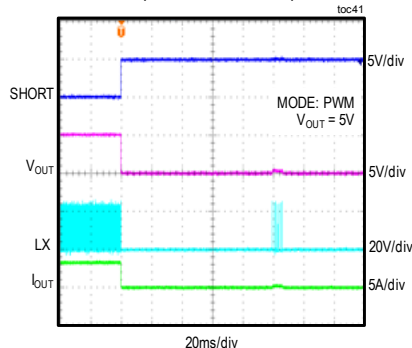
OUTPUT SHORT IN STEADY STATE (LOAD CURRENT 3A)
