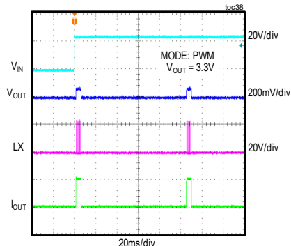
OUTPUT SHORT DURING STARTUP
