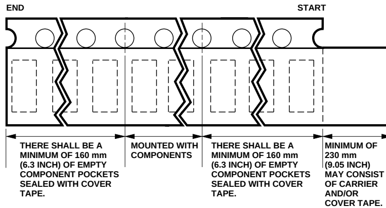
Figure 14. Tape Leader and Trailer Dimensions.
