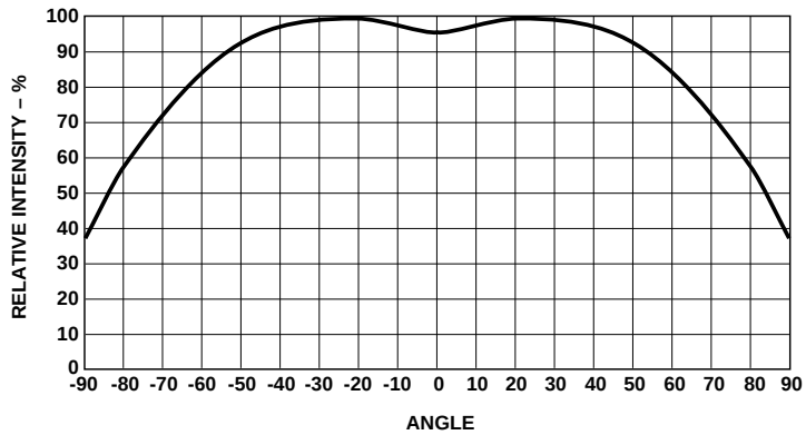
Figure 6. Relative Intensity vs. Angle for HSMB-C170 and HSMB-C190.
