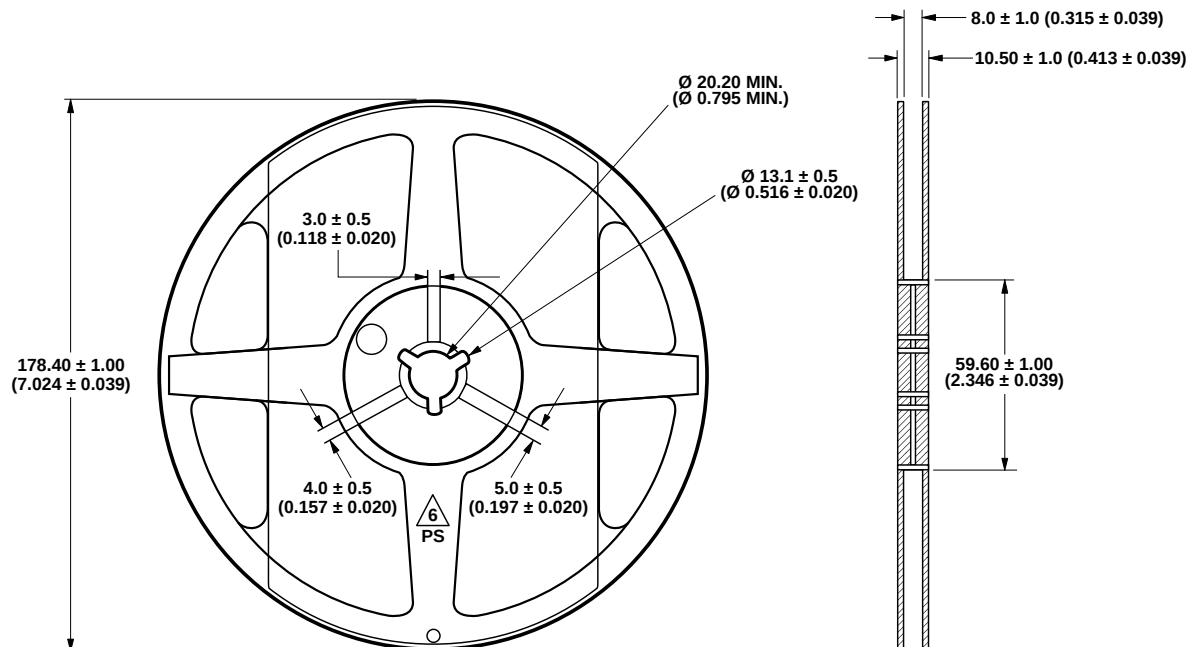
Figure 12. Reel Dimensions.
