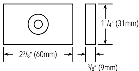
Armature Plate
