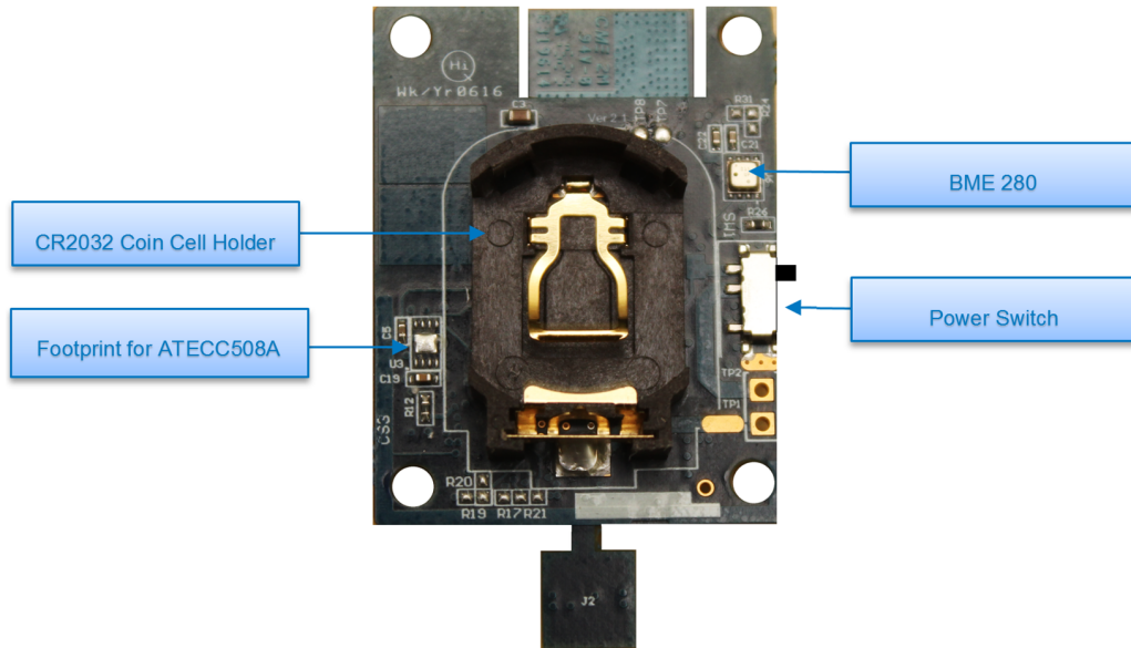
Figure 1-4. Bottom Side
