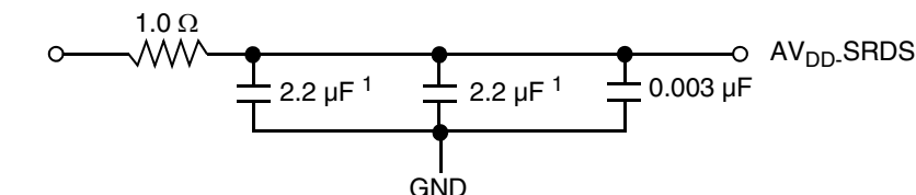
Figure 47. SerDes PLL power supply filter circuit
