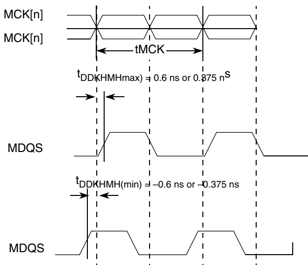
Figure 5. t_{DDKMH} timing diagram
