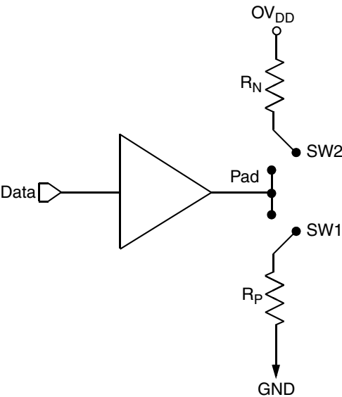
Figure 48. Driver Impedance measurement
