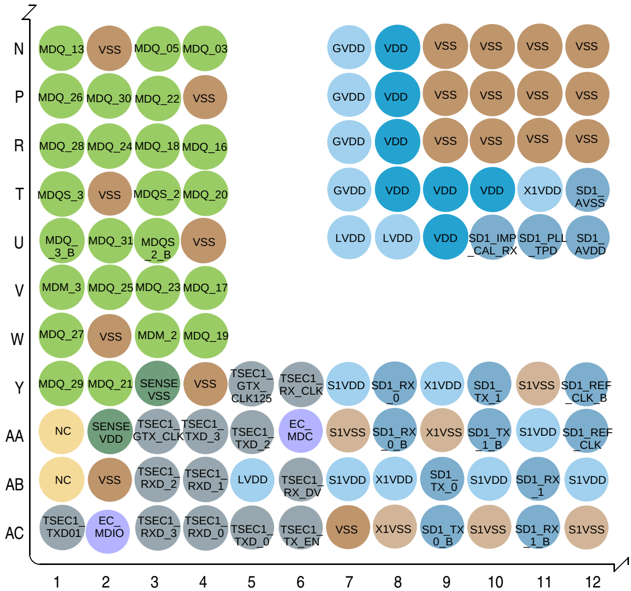
DETAIL C
