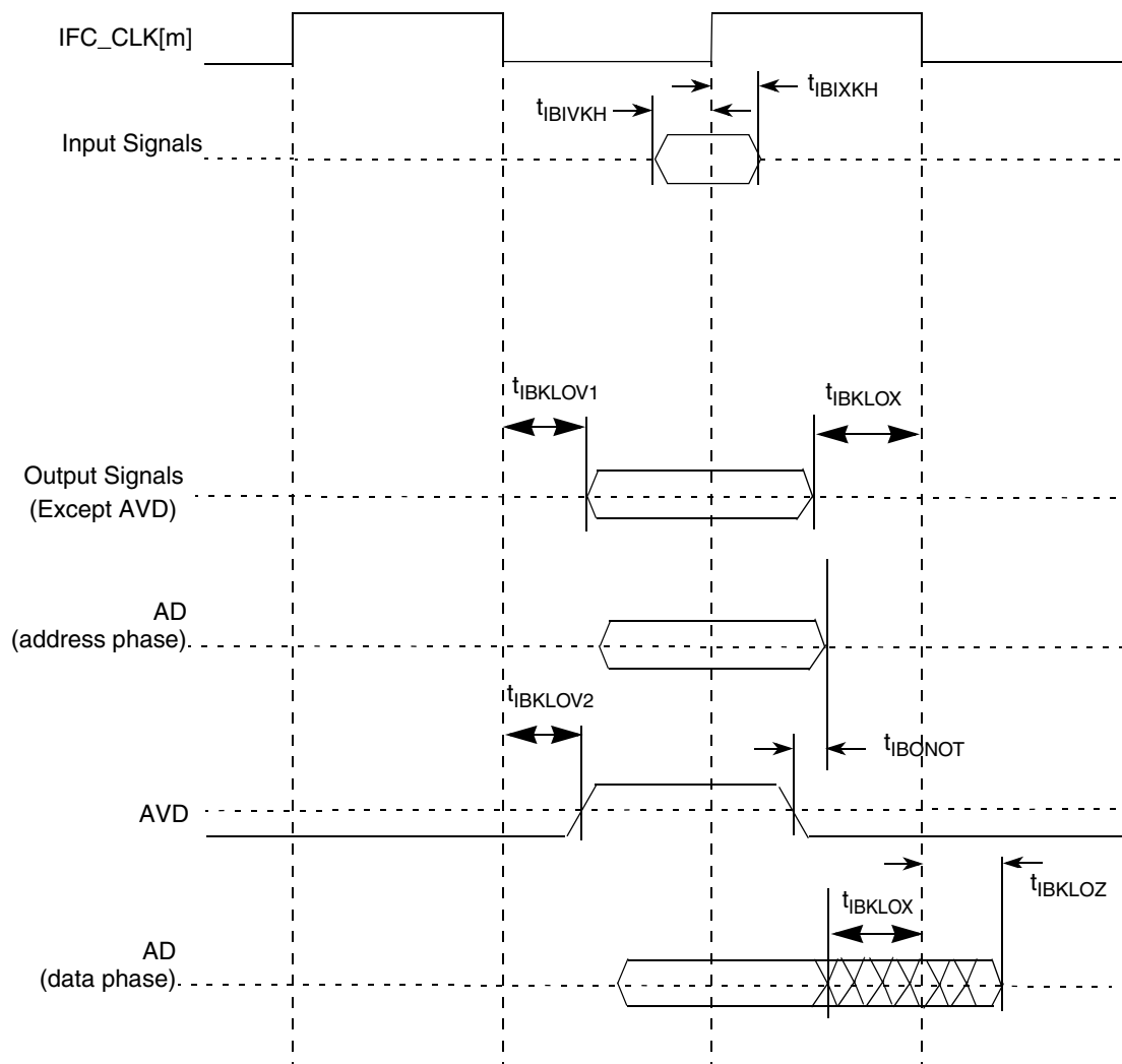
Figure 23. Integrated flash controller signals
