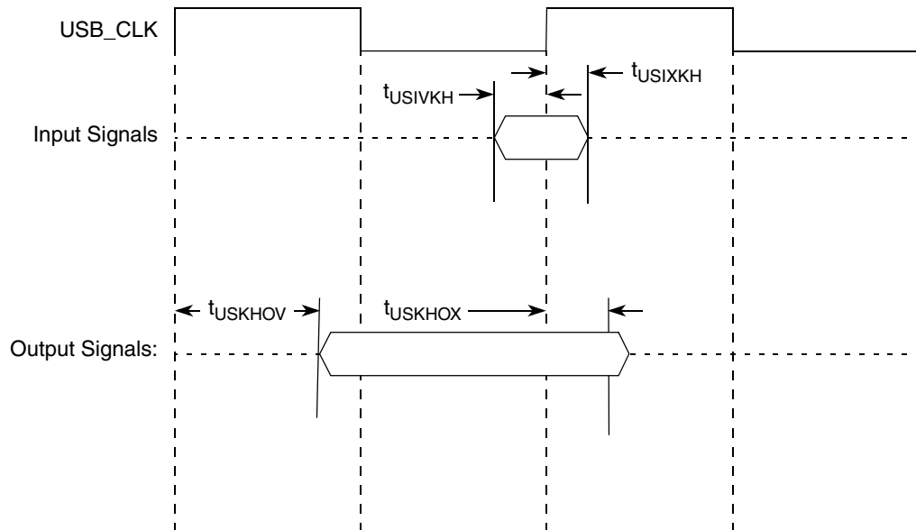
Figure 20. USB signals
