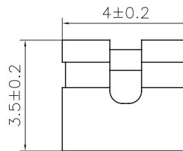
MC-2205CG (Open Type)
