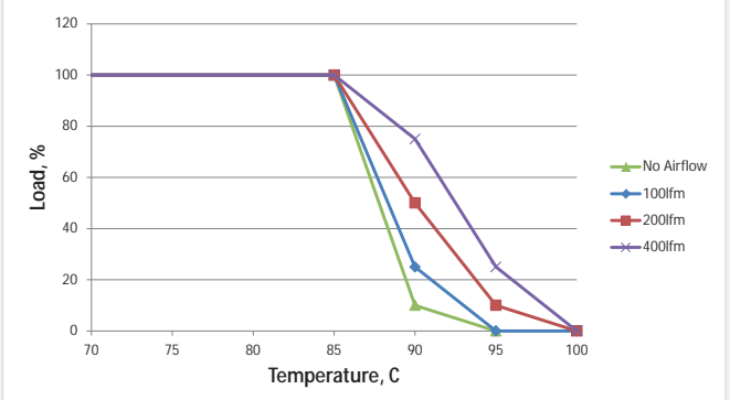
MTC1S2412MC - 36Vin
