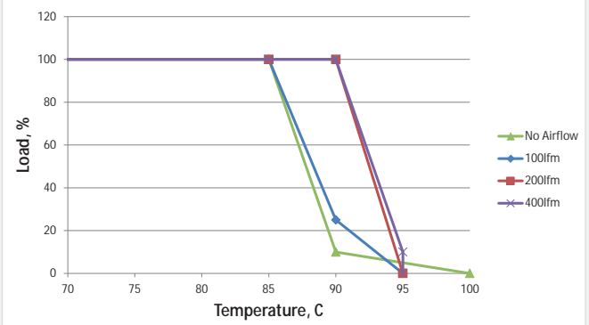
MTC1S2403MC - 36Vin
