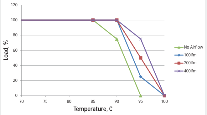
MTC1S1205MC - 18Vin
