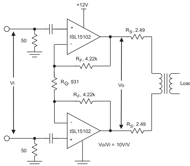
Figure 16. Passive Termination Circuit
