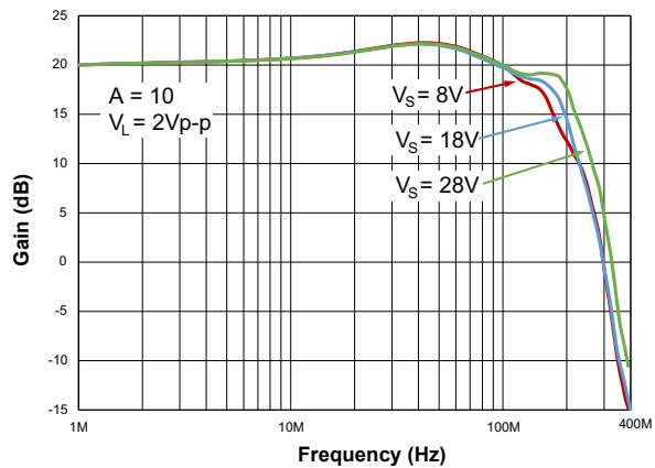
Figure 13. Small Signal Frequency Response vs Supply Voltage
