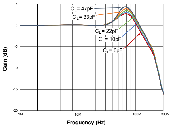
Figure 12. Common-Mode Small Signal Frequency Response vs C_{LOAD}
