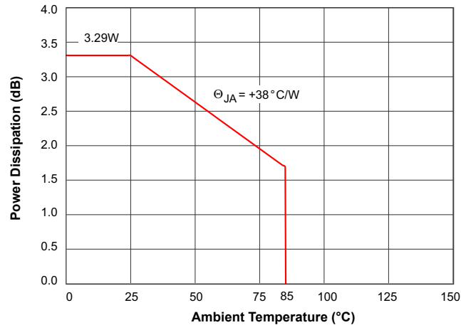
Figure 14. Package Power Dissipation vs Ambient Temperature
