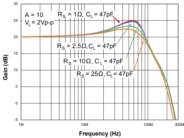
Figure 10. Small Signal Frequency Response vs R_S and C_{LOAD}
