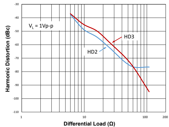
Figure 7. 4MHz Harmonic Distortion vs Load
