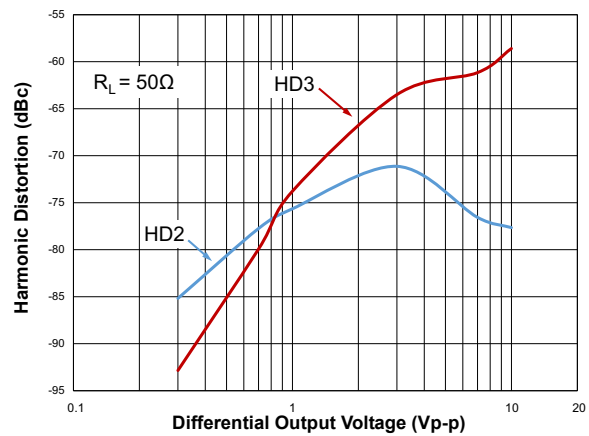
Figure 5. 4MHz Harmonic Distortion vs Output Swing
