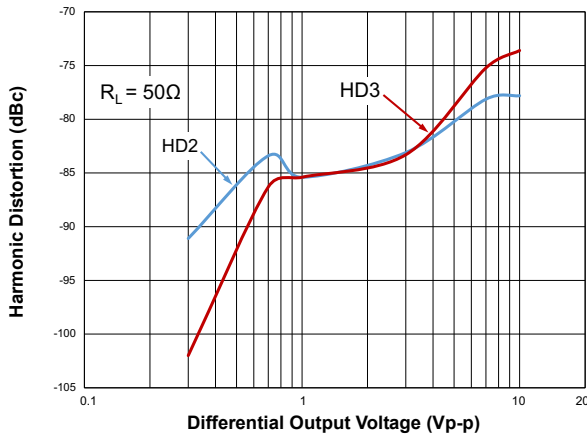
Figure 4. 1MHz Harmonic Distortion vs Output Swing
