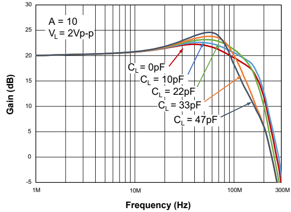
Figure 9. Small Signal Frequency Response vs C_{LOAD}
