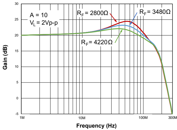
Figure 8. Small Signal Frequency Response vs R_F
