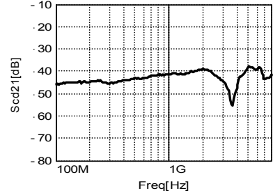
Differential mode to common mode conversion characteristic
