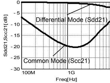
Insertion Loss
