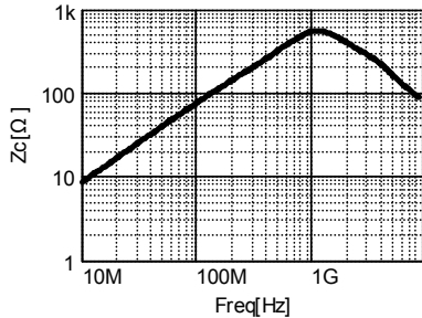
Common Mode Impedance
