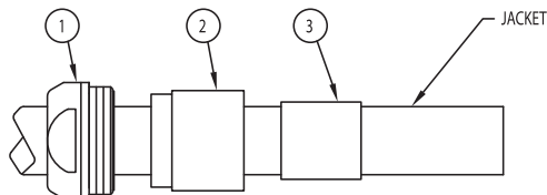
1. CUT CABLE END SQUARE. PLACE CLAMP NUT ASSEMBLY (ITEM 1), SPACER (ITEM 2) AND LARGE CRIMP SLEEVE (ITEM 3) OVER THE JACKET.
