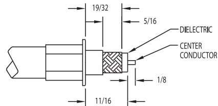
4 A. REMOVE INNER JACKET AND INNER BRAID TO 19/32 DIM. REMOVE INNER JACKET AN ADDITIONAL 5/16 EXPOSING INNER BRAID. B. REMOVE DIELECTRIC TO 11/16 DIM, AND CUT CENTER CONDUCTOR TO BE 1/8 LONG.
