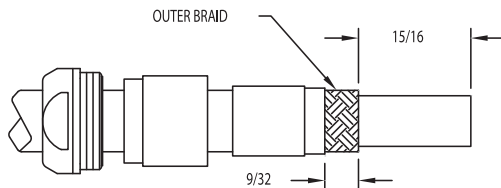
2. REMOVE JACKET AND OUTER BRAID TO 15/16 DIM. THEN REMOVE JACKET AN ADDITIONAL 9/32 EXPOSING OUTER BRAID.
