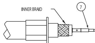
5. PLACE THE MALE OR FEMALE CONNECTOR CONTACT (ITEM 7) ON THE CABLE CENTER CONDUCTOR, BOTTOM AGAINST DIELECTRIC AND SOLDER OR CRIMP IN PLACE.
