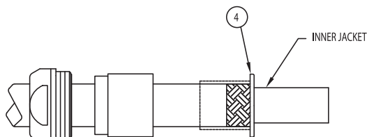
3. SLIDE K-GRIP (ITEM 4) OVER INNER JACKET AND UNDER OUTER BRAID. HOLD IN POSITION AND MOVE CRIMP SLEEVE FORWARD AGAINST SHOULDER AND CRIMP IN PLACE USING APPROPRIATE HEX DIE.
