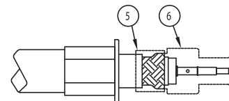
6. PLACE SMALL SLEEVE (ITEM 5) OVER INNER BRAID OF CABLE. SLIDE BODY ASSEMBLY (ITEM 6) OVER THE DIELECTRIC AND UNDER THE INNER BRAID UNTIL THE CENTER CONTACT LOCKS IN PLACE IN BODY ASSEMBLY. (NOTE; CAUTION MUST BE EXERCISED NOT TO ALLOW ANY BRAID STRANDS TO REMAIN INSIDE THE BODY ASSEMBLY. ALL BRAID MUST BE ON THE OUTSIDE OF THE BODY). SLIDE CRIMP SLEEVE FORWARD OVER BOTH THE BODY AND BRAID TO THE BODY SHOULDER. CRIMP IN PLACE. PUSH ALL LOOSE PARTS FORWARD ON CABLE AND INSERT INTO MAIN CONNECTOR BODY (ITEM 8). THREAD CLAMP NUT ASSEMBLY INTO BODY AND LOCK SECURELY.
