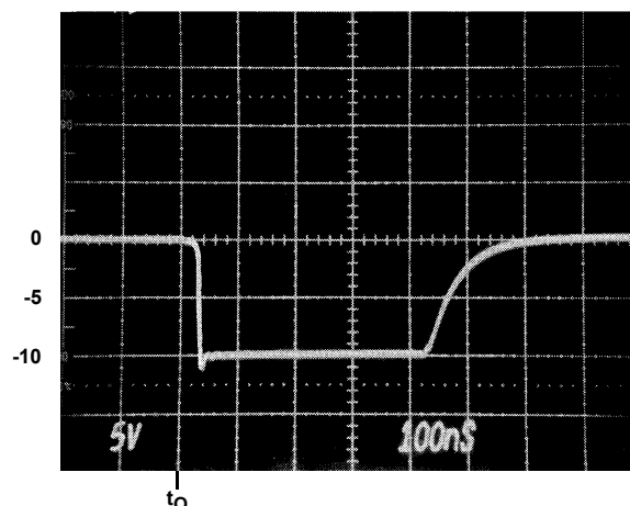
FIGURE 2F. V_{IN} = -10V
