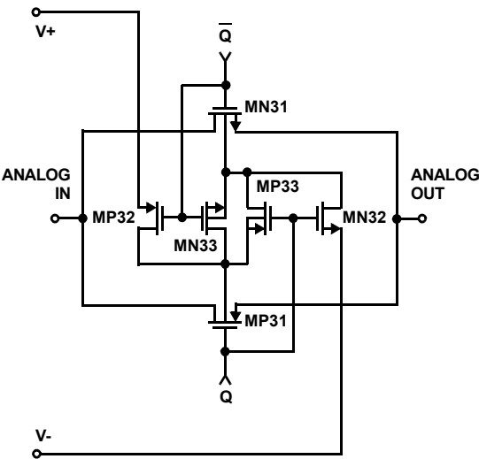
SWITCH CELL
