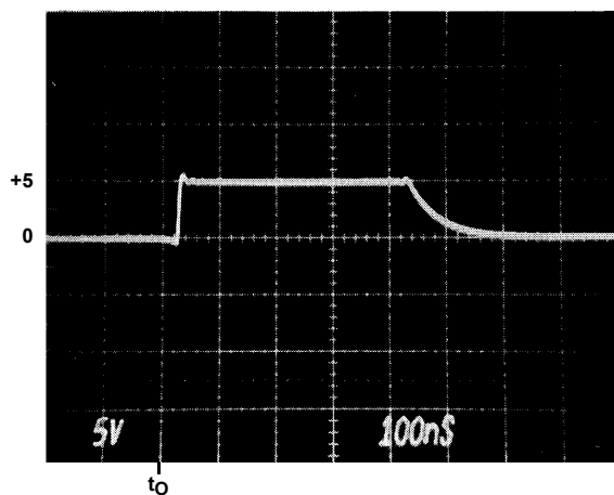
FIGURE 2C. V_{IN} = +5V
