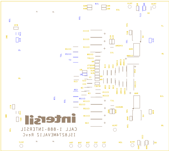
Figure 15. Silkscreen Bottom
