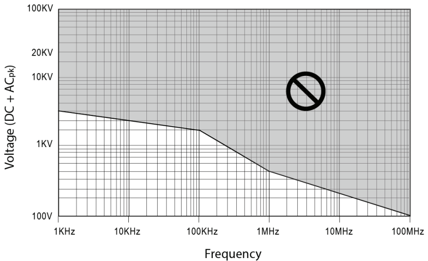
Figure 4: Voltage Derating Curve
