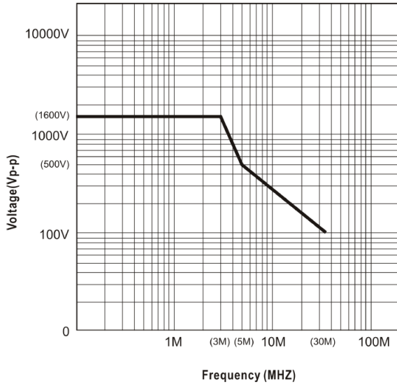
Figure 1. CT4079-NA Derating Curve
