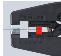
Precise stripping from 0.03 to 10 mm 2 without re-adjustment
