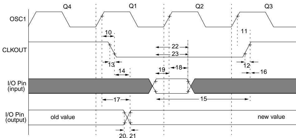
FIGURE 13-3: CLKOUT AND I/O TIMING
