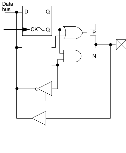
FIGURE 5-1: BLOCK DIAGRAM OF RA1:RA0 PINS
