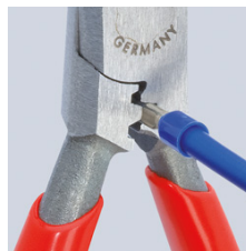
Crimping 0.5 to 2.5 mm 2
