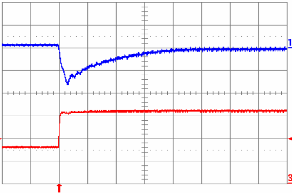
Fig. 2.5V.7: Output voltage response for V_{out} = 2.5\text{ V} to positive load current step change from 8 A to 16 A with slew rate of 5\text{ A}/\mu\text{s} at V_{in} = 5\text{ V} . Top trace: output voltage (100 mV/div.); Bottom trace: load current (5 A/div.). C_o = 100\ \mu\text{F} ceramic. Time scale: 20 \mu\text{s} /div.
