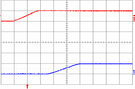
Fig. 1.0V.5: Turn-on transient for V_{out} = 1.0\text{ V} with application of V_{in} at full rated load current (resistive) and 100\ \mu\text{F} external capacitance at V_{in} = 5\text{ V} . Top trace: V_{in} (5 V/div.); Bottom trace: output voltage (1 V/div.); Time scale: 2 ms/div.
