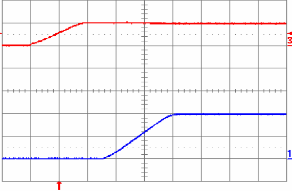
Fig. 2.0V.5: Turn-on transient for V_{out} = 2.0\text{ V} with application of V_{in} at full rated load current (resistive) and 100\mu\text{F} external capacitance at V_{in} = 5\text{ V} . Top trace: V_{in} (5 V/div.); Bottom trace: output voltage (1 V/div.); Time scale: 2 ms/div.
