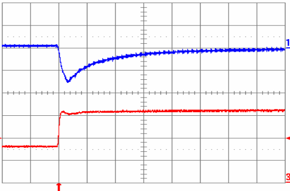
Fig. 0.7525V.7: Output voltage response for V_{out} = 0.7525 V to positive load current step change from 8 A to 16 A with slew rate of 5 \text{ A}/\mu\text{s} at V_{in} = 5 V. Top trace: output voltage (100 mV/div.); Bottom trace: load current (5 A/div.). C_o = 100 \mu\text{F} ceramic. Time scale: 20 \mu\text{s} /div.
