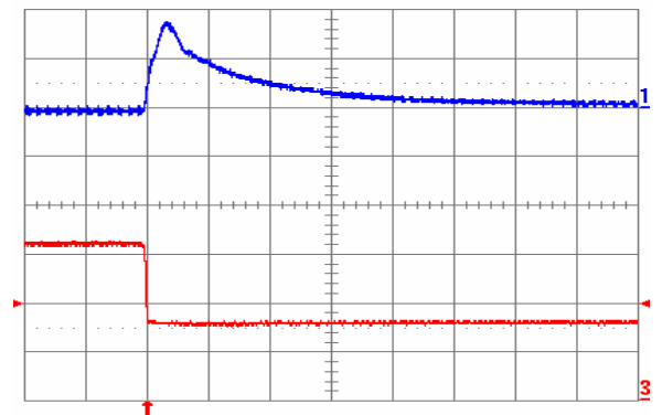
Fig. 0.7525V.8: Output voltage response for V_{out} = 0.7525 V to negative load current step change from 16 A to 8 A with slew rate of -5 \text{ A}/\mu\text{s} at V_{in} = 5 V. Top trace: output voltage (100 mV/div.); Bottom trace: load current (5 A/div.). C_o = 100 \mu\text{F} ceramic. Time scale: 20 \mu\text{s} /div.
