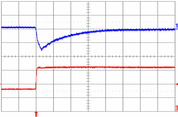
Fig. 2.0V.7: Output voltage response for V_{out} = 2.0\text{ V} to positive load current step change from 8 A to 16 A with slew rate of 5\text{ A}/\mu\text{s} at V_{in} = 5\text{ V} . Top trace: output voltage (100 mV/div.); Bottom trace: load current (5 A/div.). C_o = 100\mu\text{F} ceramic. Time scale: 20 \mu\text{s} /div.
