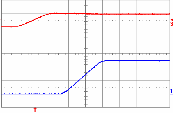
Fig. 2.5V.5: Turn-on transient for V_{out} = 2.5\text{ V} with application of V_{in} at full rated load current (resistive) and 100\ \mu\text{F} external capacitance at V_{in} = 5\text{ V} . Top trace: V_{in} (5 V/div.); Bottom trace: output voltage (1 V/div.); Time scale: 2 ms/div.
