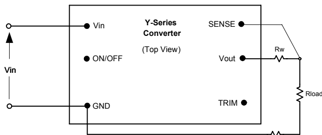
Fig. D: Remote sense circuit configuration.
