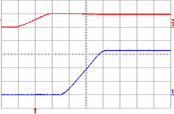
Fig. 3.3V.5: Turn-on transient for V_{out} = 3.3\text{ V} with application of V_{in} at full rated load current (resistive) and 100\ \mu\text{F} external capacitance at V_{in} = 5\text{ V} . Top trace: V_{in} (5 V/div.); Bottom trace: output voltage (1 V/div.); Time scale: 2 ms/div.
