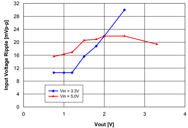
Fig. B: Input Voltage Ripple, C_{IN} = 470 \mu\text{F} polymer + 2 \times 47 \mu\text{F} ceramic.
