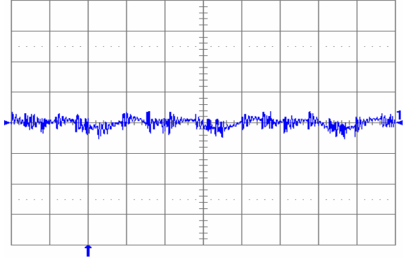
Fig. 1.0V.6: Output voltage ripple (20 mV/div.) at full rated load current into a resistive load with external capacitance 100\ \mu\text{F} ceramic + 1\ \mu\text{F} ceramic and V_{in} = 5\text{ V} for V_{out} = 1.0\text{ V} . Time scale: 2 \mu\text{s} /div.
