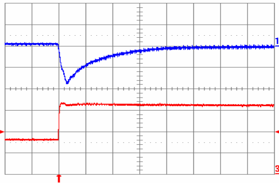
Fig. 1.5V.7: Output voltage response for V_{out} = 1.5\text{ V} to positive load current step change from 8 A to 16 A with slew rate of 5\text{ A}/\mu\text{s} at V_{in} = 5\text{ V} . Top trace: output voltage (100 mV/div.); Bottom trace: load current (5 A/div.). C_o = 100\ \mu\text{F} ceramic. Time scale: 20 \mu\text{s} /div.
