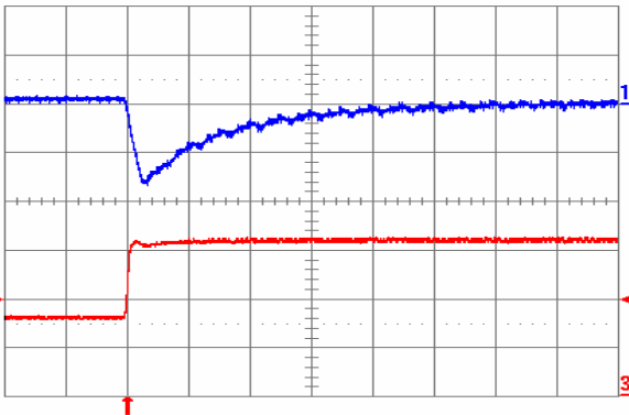
Fig. 1.2V.6: Output voltage response for V_{out} = 1.2\text{ V} to positive load current step change from 8 A to 16 A with slew rate of 5\text{ A}/\mu\text{s} at V_{in} = 5\text{ V} . Top trace: output voltage (100 mV/div.); Bottom trace: load current (5 A/div.). C_o = 100\ \mu\text{F} ceramic. Time scale: 20 \mu\text{s} /div.
