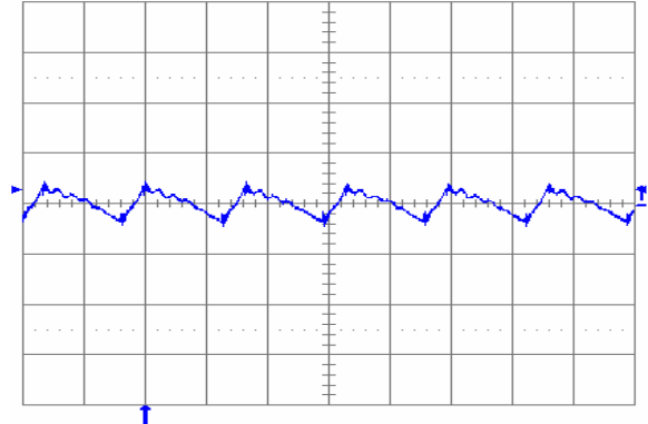
Fig. 2.5V.6: Output voltage ripple (20 mV/div.) at full rated load current into a resistive load with external capacitance 100\text{ }\mu\text{F} ceramic + 1\text{ }\mu\text{F} ceramic, and V_{in} = 12\text{ V} for V_{out} = 2.5\text{ V} . Time scale: 2 \mu\text{s} /div.
