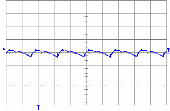
Fig. 1.8V.6: Output voltage ripple (20 mV/div.) at full rated load current into a resistive load with external capacitance 100\ \mu\text{F} ceramic + 1\ \mu\text{F} ceramic, and V_{in} = 12\text{ V} for V_{out} = 1.8\text{ V} . Time scale: 2 \mu\text{s} /div.
