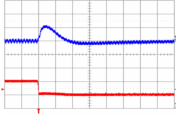
Fig. 1.5V.8: Output voltage response for V_{out} = 1.5\text{ V} to negative load current step change from 10 A to 5 A with slew rate of -5\text{ A}/\mu\text{s} at V_{in} = 12\text{ V} . Top trace: output voltage (100 mV/div.); Bottom trace: load current (2 A/div.). C_o = 100\ \mu\text{F} ceramic. Time scale: 20 \mu\text{s} /div.
