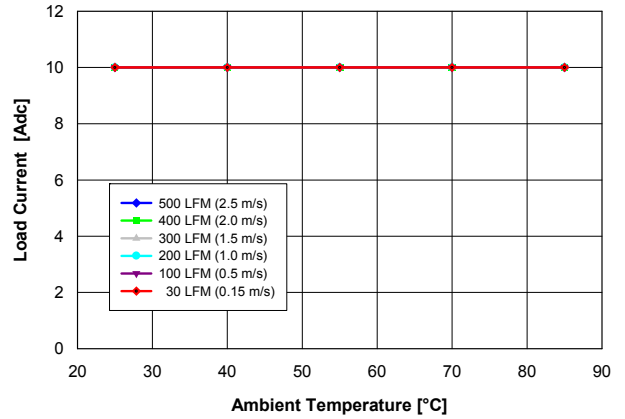
Fig. 1.8V.2: Available load current vs. ambient temperature and airflow rates for V out = 1.8 V converter mounted horizontally with V in = 12 V, and maximum MOSFET temperature ≤ 110 °C.
