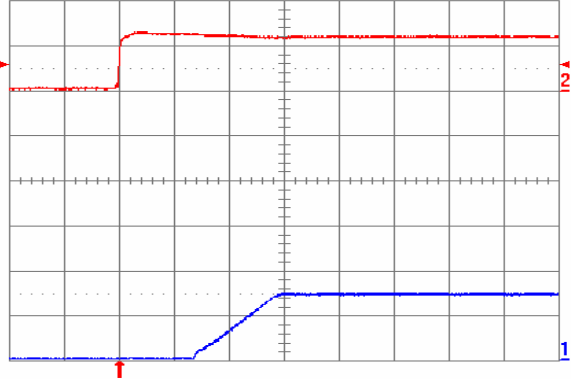
Fig. 1.5V.5: Turn-on transient for V_{out} = 1.5\text{ V} with application of V_{in} at full rated load current (resistive) and 100\ \mu\text{F} external capacitance at V_{in} = 12\text{ V} . Top trace: V_{in} (10 V/div.); Bottom trace: output voltage (1 V/div.); Time scale: 2 ms/div.
