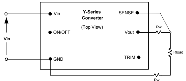
Fig. B: Circuit configuration for ON/OFF function.
