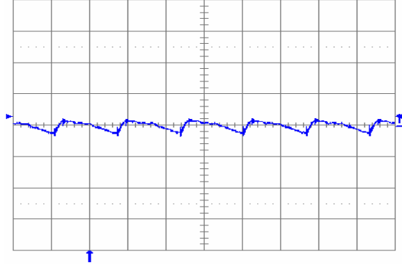
Fig. 1.5V.6: Output voltage ripple (20 mV/div.) at full rated load current into a resistive load with external capacitance 100\ \mu\text{F} ceramic + 1\ \mu\text{F} ceramic, and V_{in} = 12\text{ V} for V_{out} = 1.5\text{ V} . Time scale: 2 \mu\text{s} /div.
