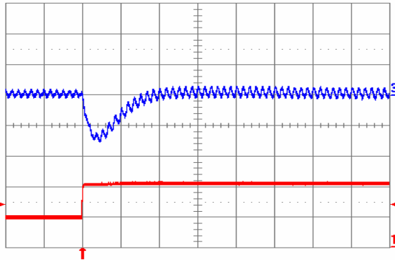
Fig. 5.0V.7: Output voltage response for V_{out} = 5.0 V to positive load current step change from 5 A to 10 A with slew rate of 5 \text{ A}/\mu\text{s} at V_{in} = 12 V. Top trace: output voltage (100 mV/div.); Bottom trace: load current (5 A/div.). C_o = 100 \mu\text{F} ceramic. Time scale: 20 \mu\text{s} /div.
