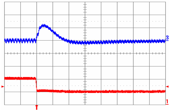
Fig. 1.8V.8: Output voltage response for V_{out} = 1.8\text{ V} to negative load current step change from 10 A to 5 A with slew rate of -5\text{ A}/\mu\text{s} at V_{in} = 12\text{ V} . Top trace: output voltage (100 mV/div.); Bottom trace: load current (5 A/div.). C_o = 100\ \mu\text{F} ceramic. Time scale: 20 \mu\text{s} /div.
