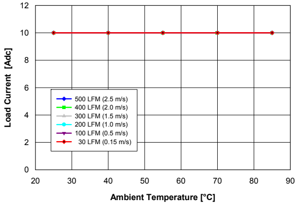
Fig. 1.8V.1: Available load current vs. ambient temperature and airflow rates for V out = 1.8 V converter mounted vertically with V in = 12 V, and maximum MOSFET temperature ≤ 110 °C.
