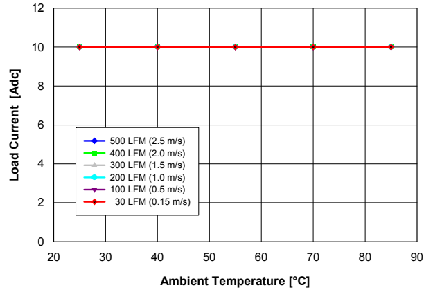
Fig. 1.5V.2: Available load current vs. ambient temperature and airflow rates for Vout = 1.5 V converter mounted horizontally with Vin = 12 V, and maximum MOSFET temperature ≤ 110 °C.
