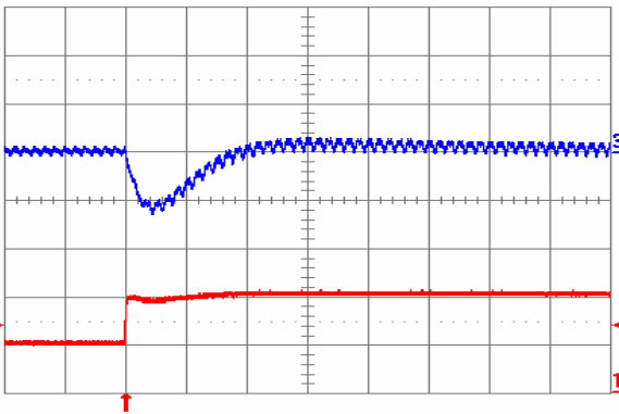
Fig. 1.8V.7: Output voltage response for V_{out} = 1.8\text{ V} to positive load current step change from 5 A to 10 A with slew rate of 5\text{ A}/\mu\text{s} at V_{in} = 12\text{ V} . Top trace: output voltage (100 mV/div.); Bottom trace: load current (5 A/div.). C_o = 100\ \mu\text{F} ceramic. Time scale: 20 \mu\text{s} /div.
