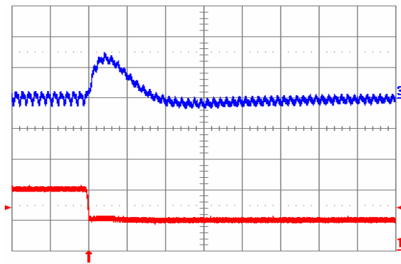
Fig. 3.3V.8: Output voltage response for V_{out} = 3.3 V to negative load current step change from 10 A to 5 A with slew rate of -5 \text{ A}/\mu\text{s} at V_{in} = 12 V. Top trace: output voltage (100 mV/div.); Bottom trace: load current (2 A/div.). C_o = 100 \mu\text{F} ceramic. Time scale: 20 \mu\text{s} /div.
