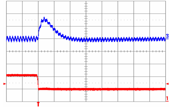
Fig. 5.0V.8: Output voltage response for V_{out} = 5.0 V to negative load current step change from 10 A to 5 A with slew rate of -5 \text{ A}/\mu\text{s} at V_{in} = 12 V. Top trace: output voltage (100 mV/div.); Bottom trace: load current (5 A/div.). C_o = 100 \mu\text{F} ceramic. Time scale: 20 \mu\text{s} /div.
