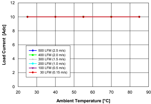
Fig. 1.5V.1: Available load current vs. ambient temperature and airflow rates for Vout = 1.5 V converter mounted vertically with Vin = 12 V, and maximum MOSFET temperature ≤ 110 °C.
