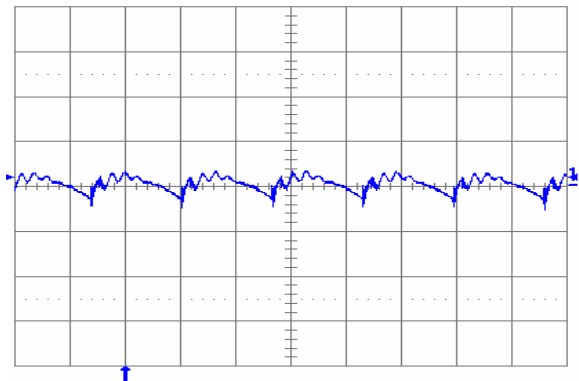
Fig. 1.0V.5: Output voltage ripple (20mV/div.) at full rated load current into a resistive load with external capacitance 100\mu F ceramic + 1\mu F ceramic and V_{in} = 12V for V_{out} = 1.0V . Time scale: 2\mu s /div.
