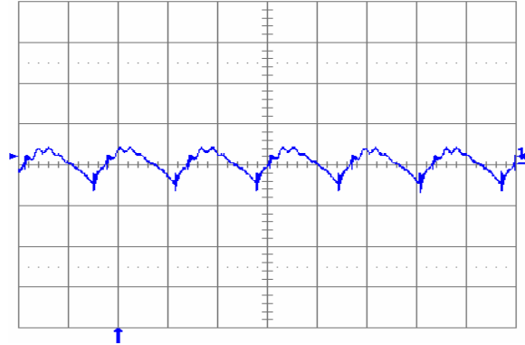
Fig. 1.8V.5: Output voltage ripple (20mV/div.) at full rated load current into a resistive load with external capacitance 100\mu F ceramic + 1\mu F ceramic and V_{in} = 12V for V_{out} = 1.8V . Time scale: 2\mu s /div.
