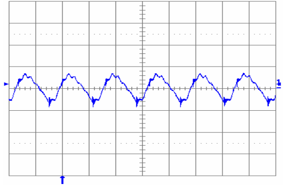
Fig. 3.3V.5: Output voltage ripple (20mV/div.) at full rated load current into a resistive load with external capacitance 100\mu F ceramic + 1\mu F ceramic and V_{in} = 12V for V_{out} = 3.3V . Time scale: 2μs/div.
