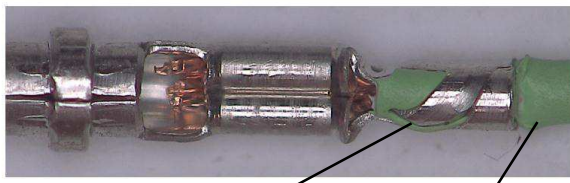
Skewing of Wire Insulation Acceptable
