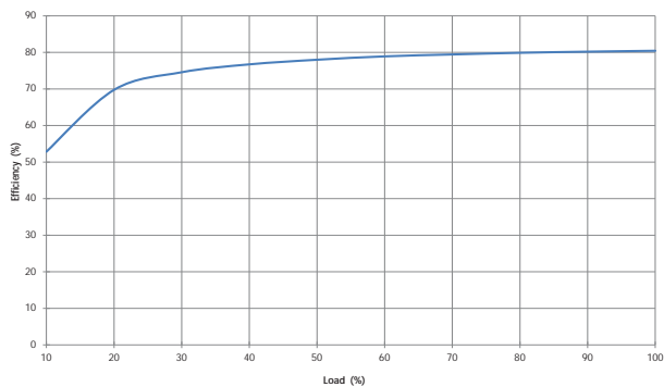
MGJ3T24150505MC
