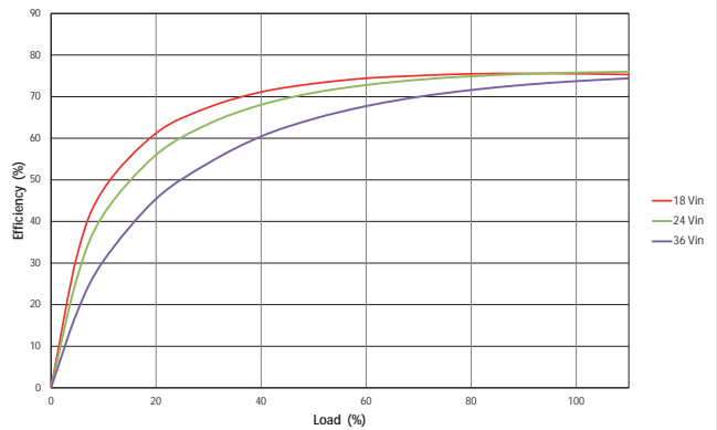
MTC1S2403MC
