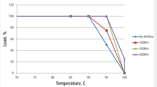
MTC1S2403MC - 18Vin
