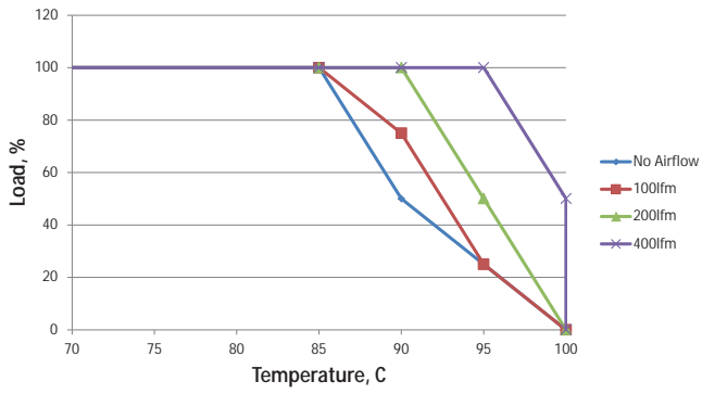
MTC1S1203MC - 9Vin
