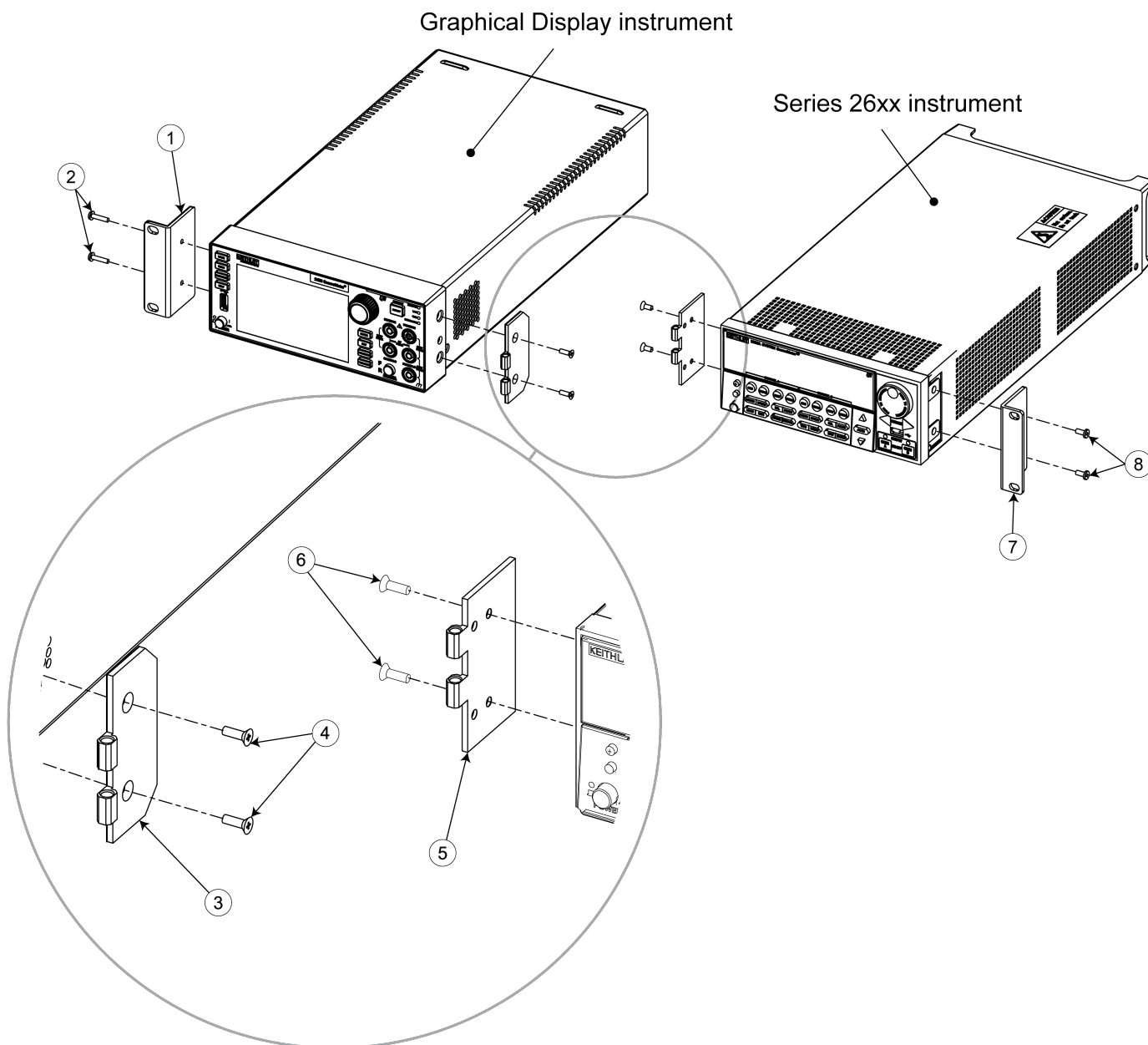
Figure 11: Install mounting hardware on the instruments
