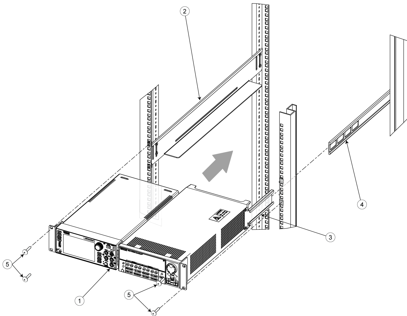
Figure 14: Install the instrument assembly in the rack
