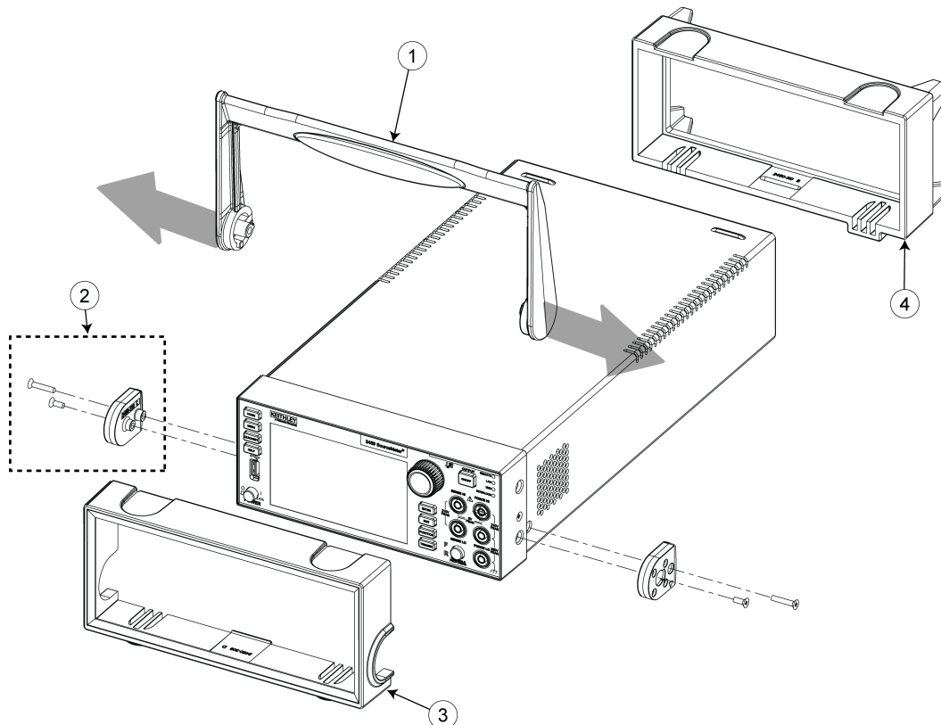
Figure 6: Remove handle and bumpers
