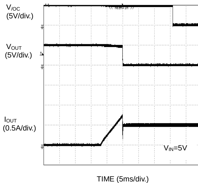
Figure 32. Over-Current Response
