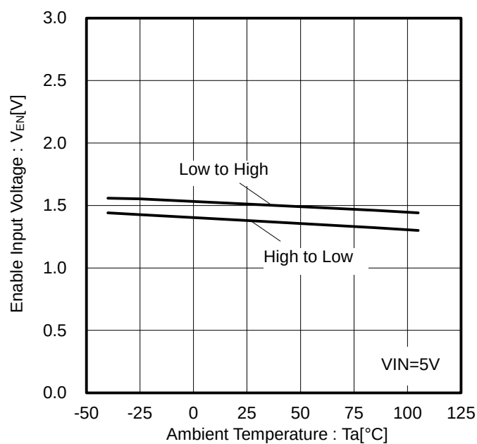
Figure 8. EN Input Voltage vs Ambient Temperature ( V_{ENH} , V_{ENL} )
