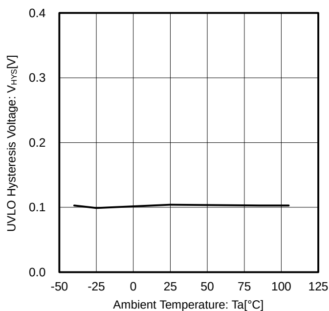
Figure 18. UVLO Hysteresis Voltage vs Ambient Temperature
