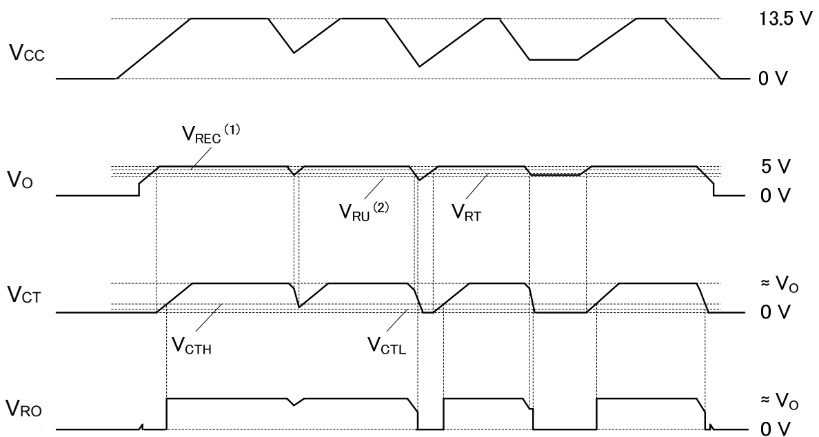
Figure 21. Timing Chart
