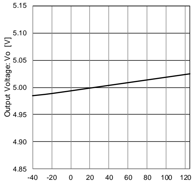
Figure 18. Output Voltage Temperature Characteristic
