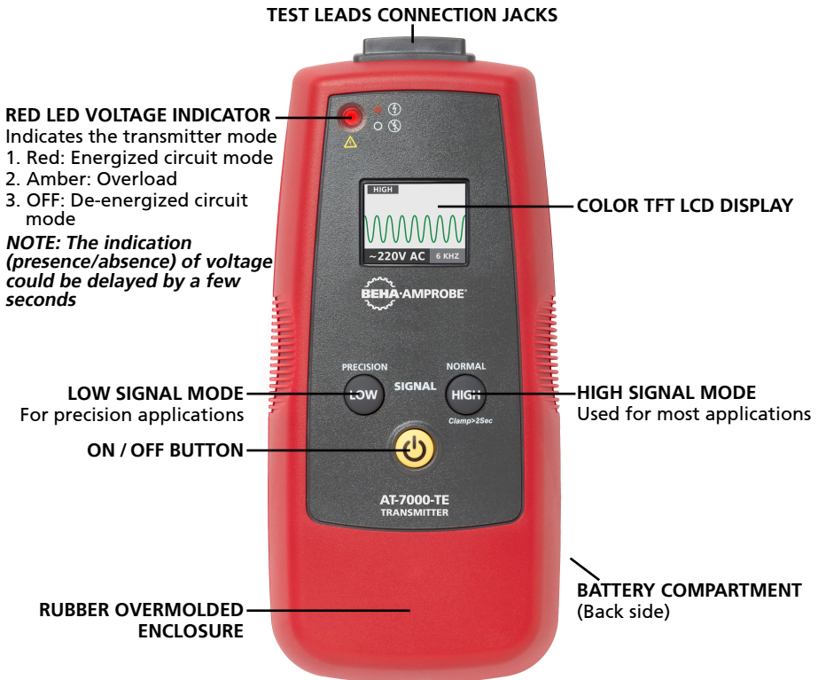
Figure 2: Overview of AT-7000-TE Transmitter
