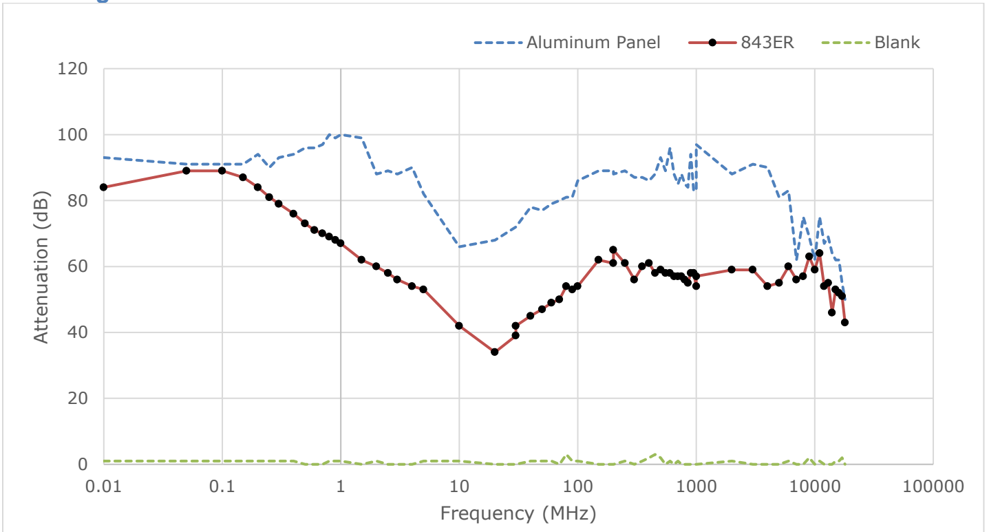
Figure 1. Attenuation of 843ER coating at different frequencies
