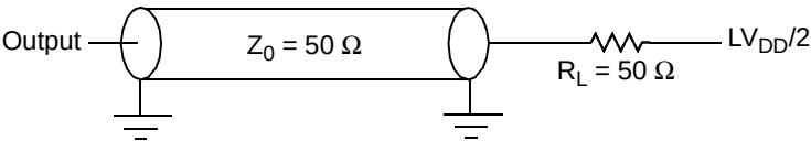
Figure 19. eTSEC AC Test Load
