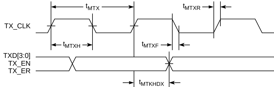
Figure 15. MII Transmit AC Timing Diagram
