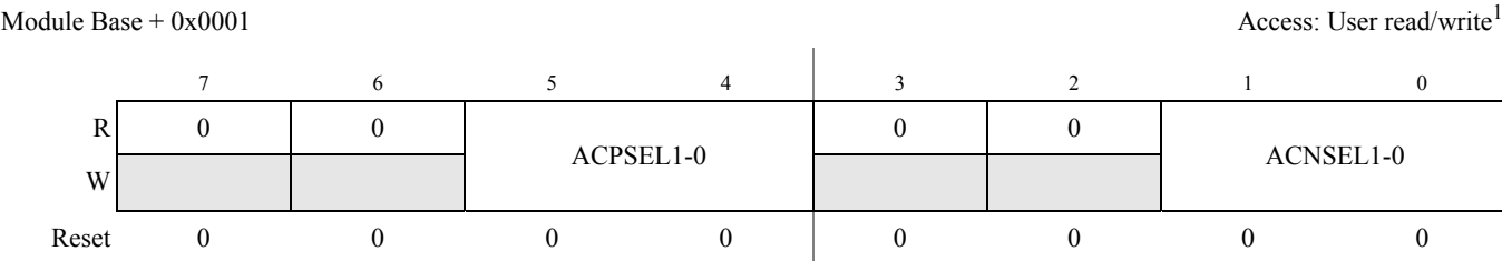
Figure 20-3. ACMP Control Register (ACMPC1)
