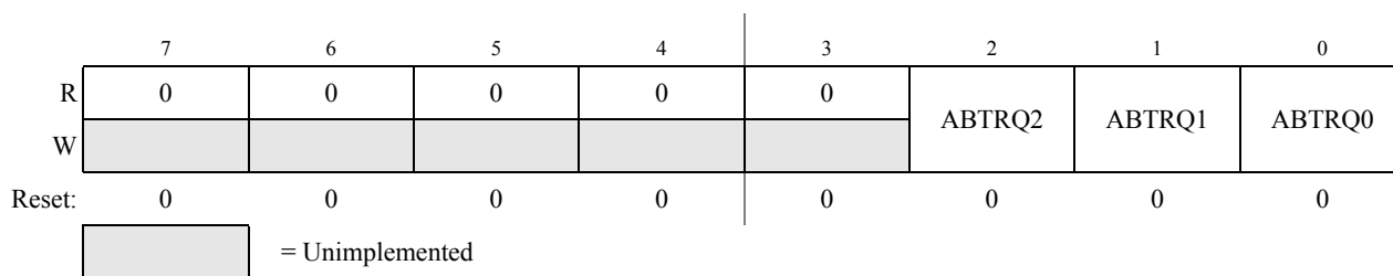
Figure 18-12. MSCAN Transmitter Message Abort Request Register (CANTARQ)
