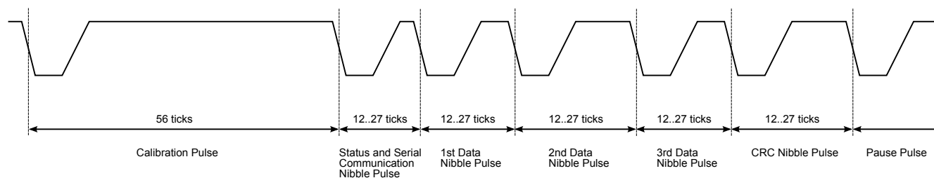
Figure 21-2. SENT Message Format
