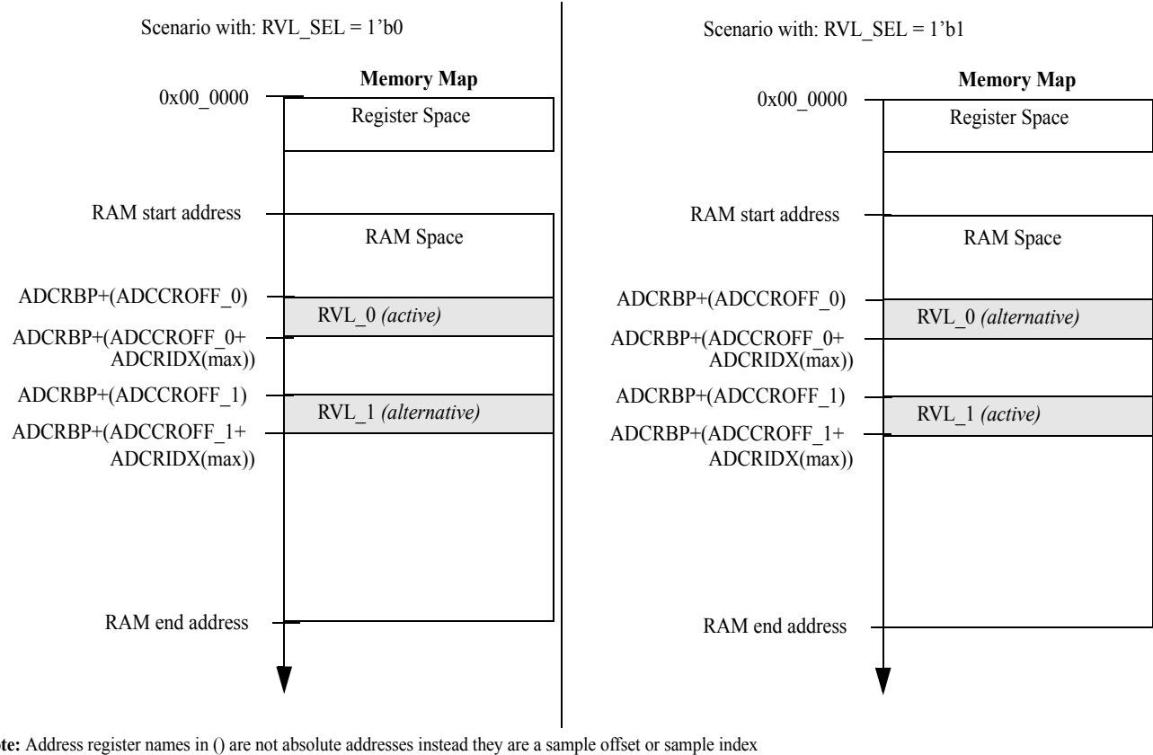
Figure 9-33. Result Value List Schema in Double Buffer Mode
