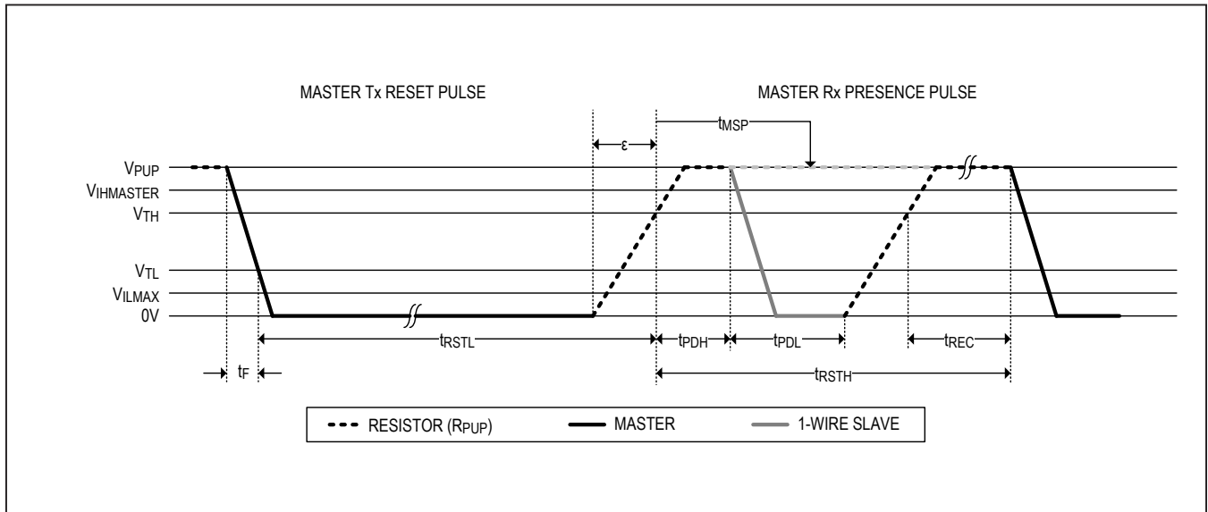
Figure 3. Initialization Procedure: Reset and Presence Pulse
