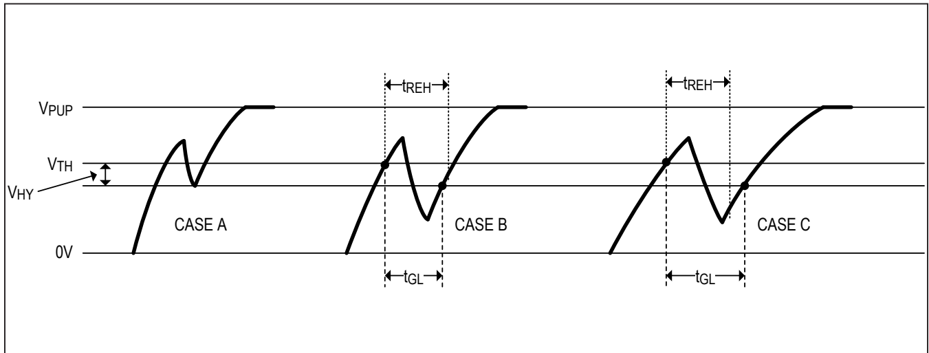
Figure 7. Noise Suppression Scheme
