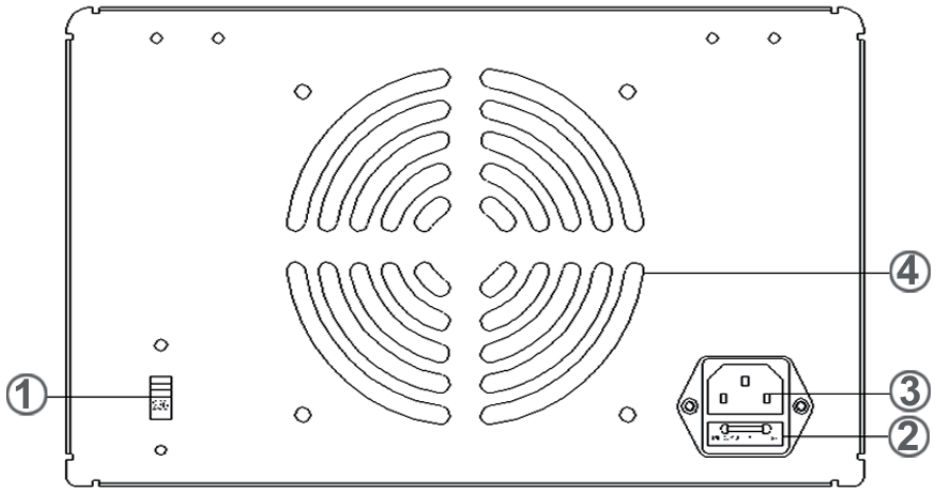
Figure 3 – Rear Panel: Models UTP3303 / 72-13610
