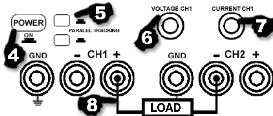
Figure 9 - Parallel Connection of the adjustable power supplies of the 72-13600 and 72-13610
