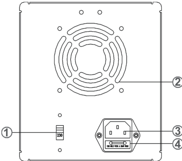
Figure 4 – Rear Panel: Models UTP1303 / 72-13610
