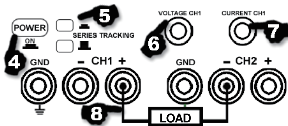
Figure 10 - Series Operation Mode of the adjustable power supplies of the models 72-13600 and 72-13610.
