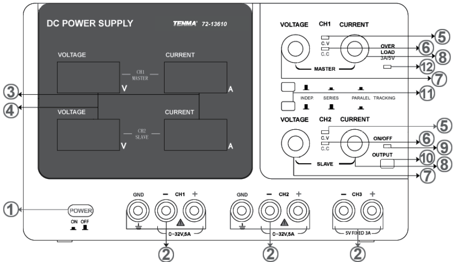
Figure 1 – Front Panel: Models 72-13600 / 72-13610
