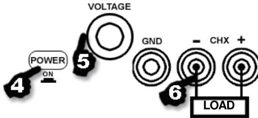
Figure 8 - Models UTP1303 and UTP1305 or each one of the adjustable power supplies of the Models 72-13600 and 72-13610 Connection.
