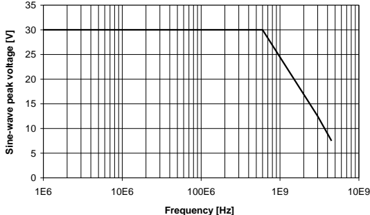
Maximum nondestructive sine-wave peak voltage versus frequency.
