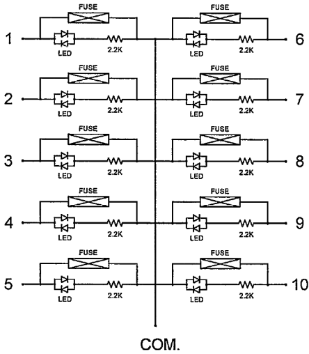
Circuit Diagram
