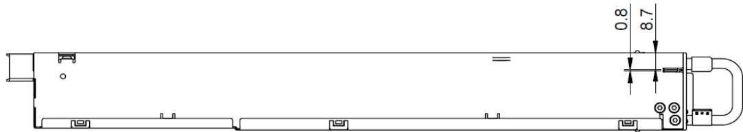
Figure 44. Side View 2
