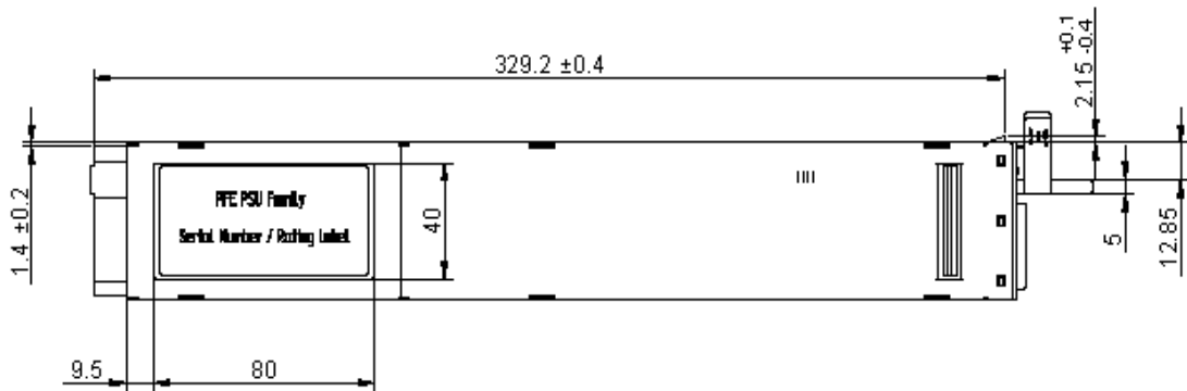
Figure 43. Top View
