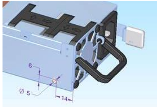
Figure 53. Polarizing screw
