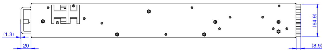
Figure 10. Bottom view
