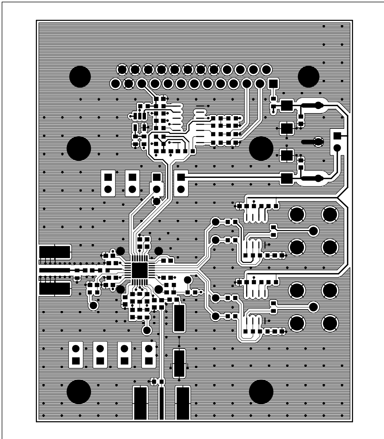
Figure 3. MAX2112 EV Kit PCB Layout—Top
