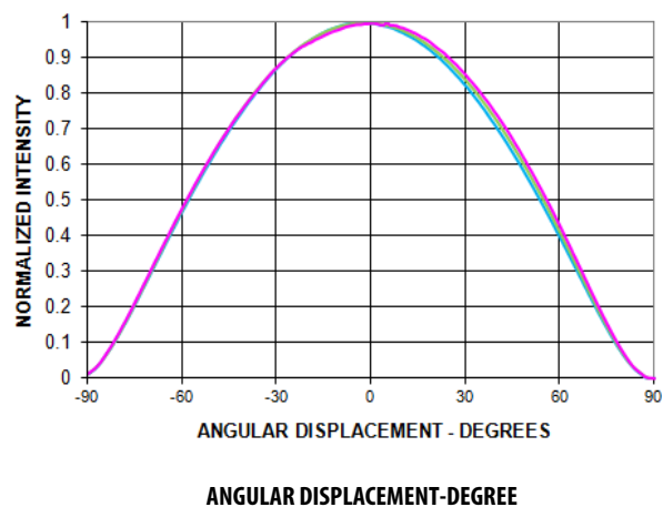
Figures 11a. Radiation pattern along x-axis of the package
